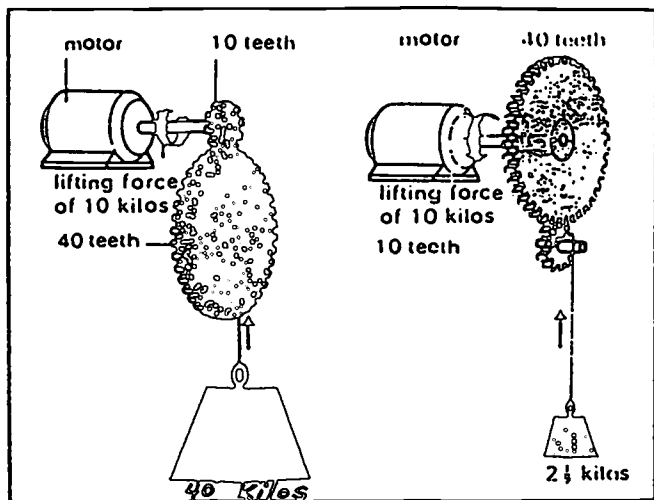
Fig. 1: In this machine, the smaller wheel, the pinion, has only a quarter as many teeth as the larger, so it will turn four times as fast. The left-hand machine will lift the heavier weight. When the positions are reversed, only a smaller weight can be lifted, but at a greater speed.
