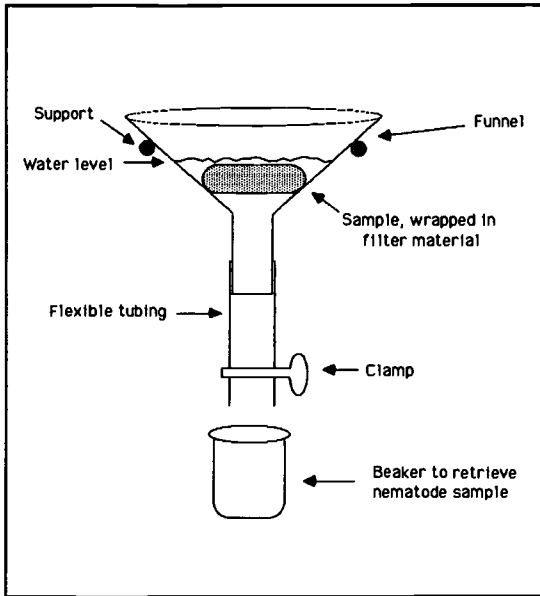
Top: Figure 8D.2. A Baermann funnel for extracting nematodes from soil. Bottom: Figure 8D.3. A dissecting microscope with transmitted light source.
