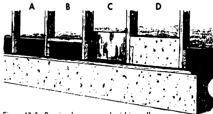
Figure 12-2. Barriers between and within walls
