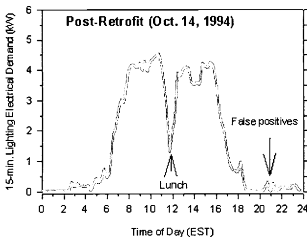
Figure 1. Sample Daily Load Profiles for Building 200
