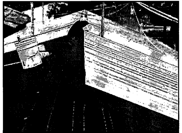
Figure 2. Reflective white metal roof that replaced the gray asphalt shingle roof. The black felt is fastened to the decking and then the 5-V crimp panels are fastened.
