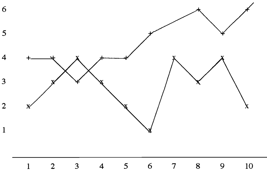
Figure 5 Scatter plots of two letter writers
