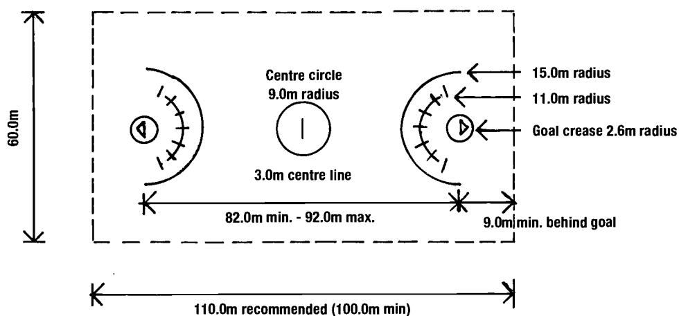
Fig. 42 Full-size women's and girls' lacrosse pitch
