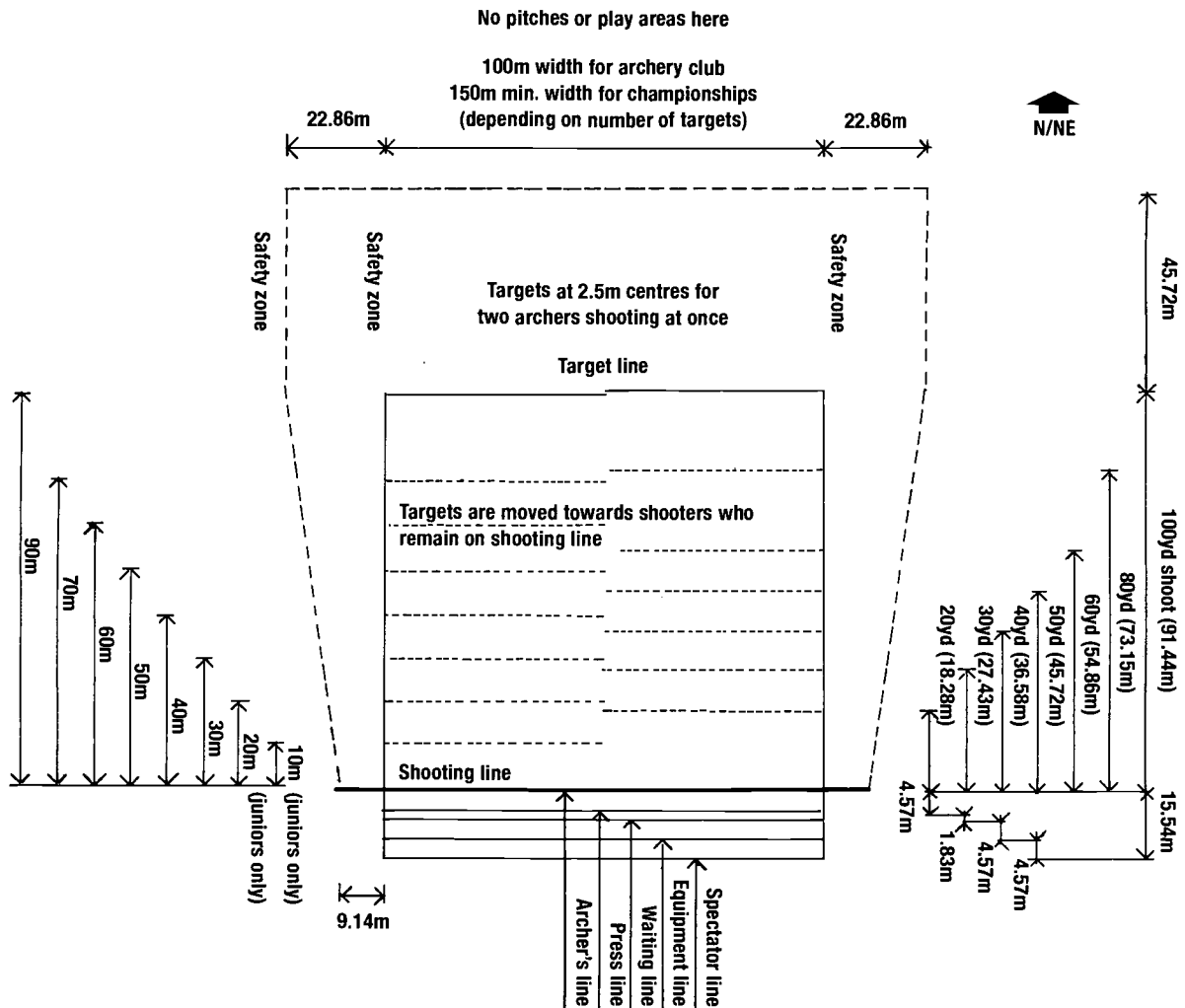
Fig. 35 Target archery range
