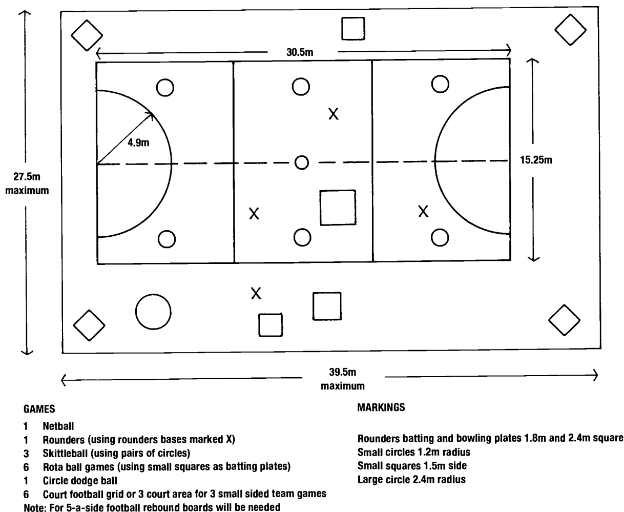
Fig. 12 Junior games court for 8-11 year olds
