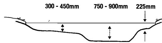
POND SECTION A-A
