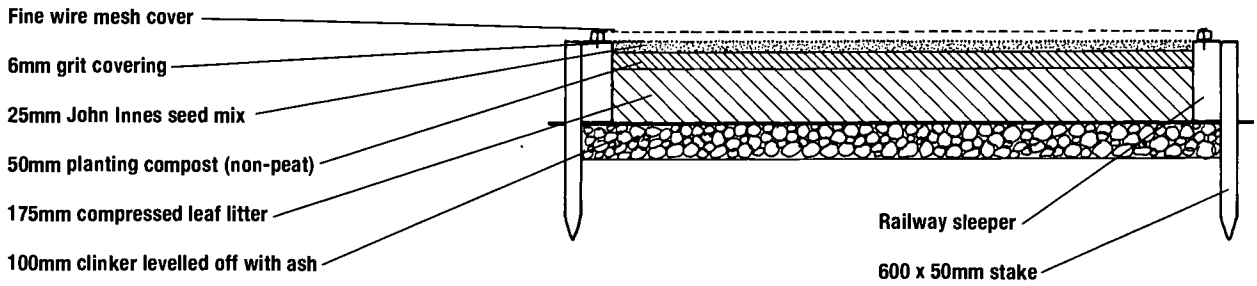
Fig. 9 Detail of a tree nursery bed
