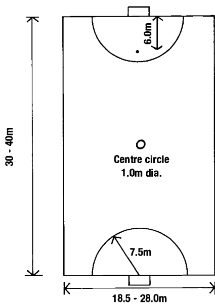
b) 5-a-side pitch
