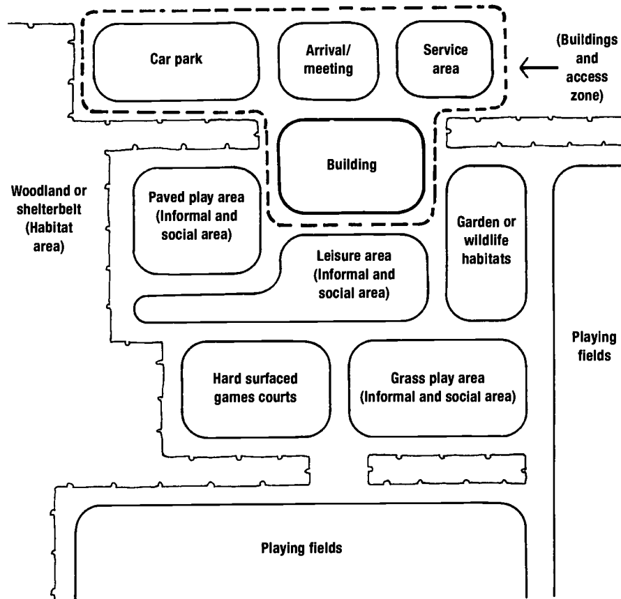
Fig. 23 Zoning of outdoor uses to improve security and safety (similar activities are grouped for better supervision)
