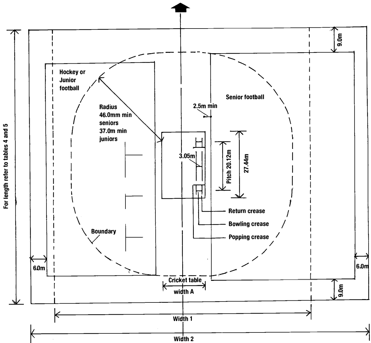
Fig. 39 Cricket square and field combined with winter games pitches
