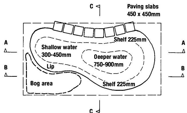
POND PLAN
