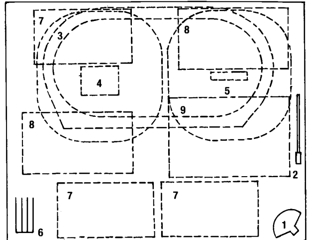
Six form entry mixed secondary school for 900 pupils aged 11-16 years 40,000m 2 all grass
