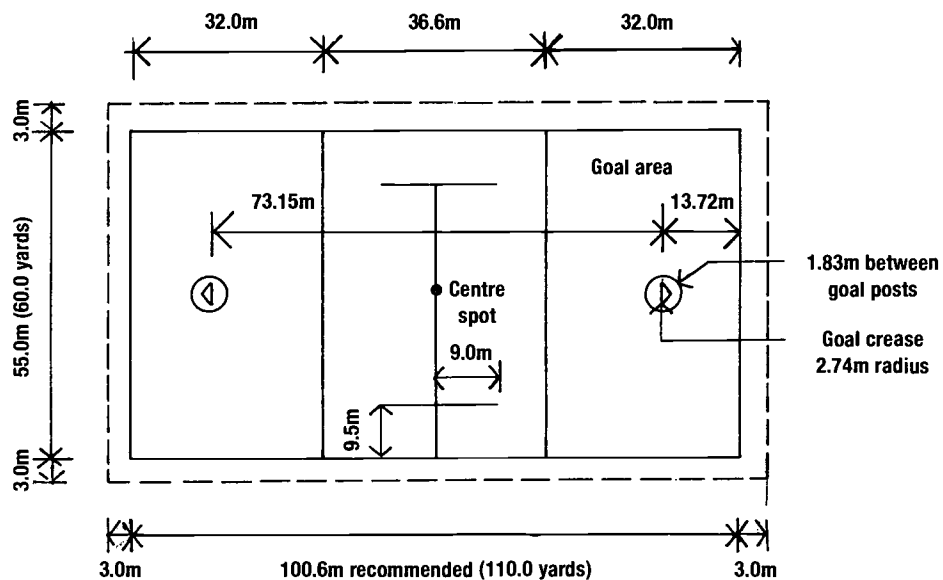
Fig. 41 Full-size men's lacrosse pitch
