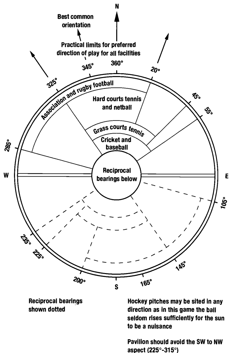
Fig. 13 Pitch orientation in relation to aspect National Playing Fields Association
