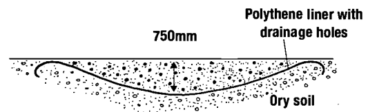
BOG AREA SECTION IN DETAIL
