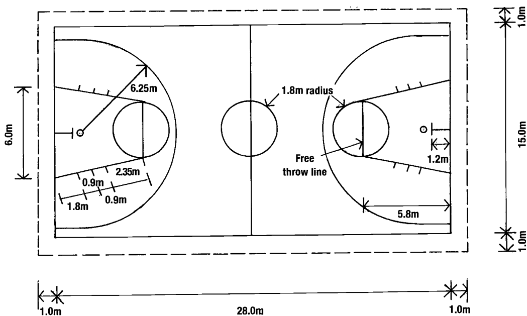
a) Full-size basketball court
