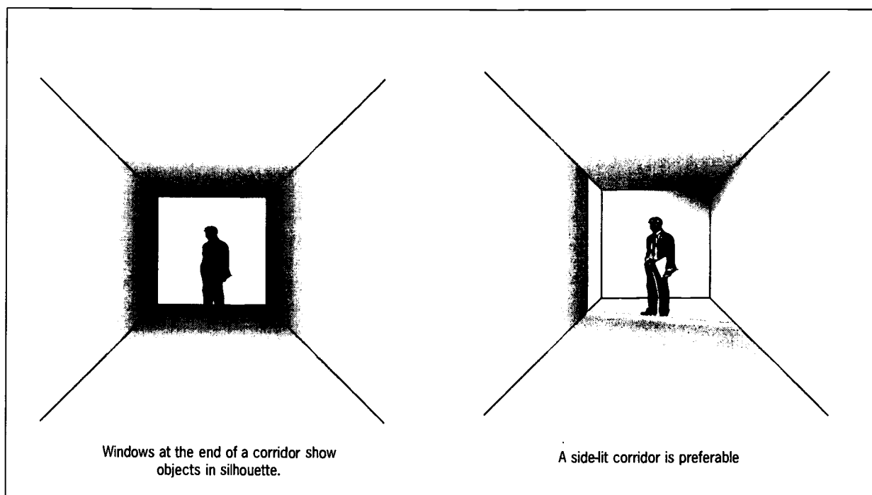
Figure 34: The benefit of a side-lit corridor.
