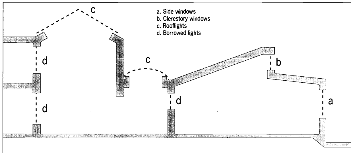
Figure 8: Window types.
