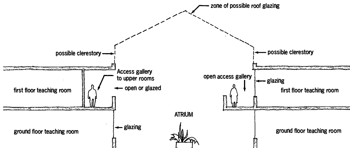
DIAGRAM SHOWING POSSIBLE SECTION THROUGH TYPICAL 2-STOREY SCHOOL ATRIUM
