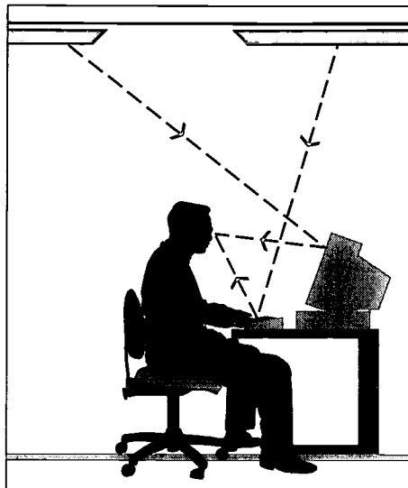
Figure 25: Veiling reflections on vertical and horizontal surfaces.
