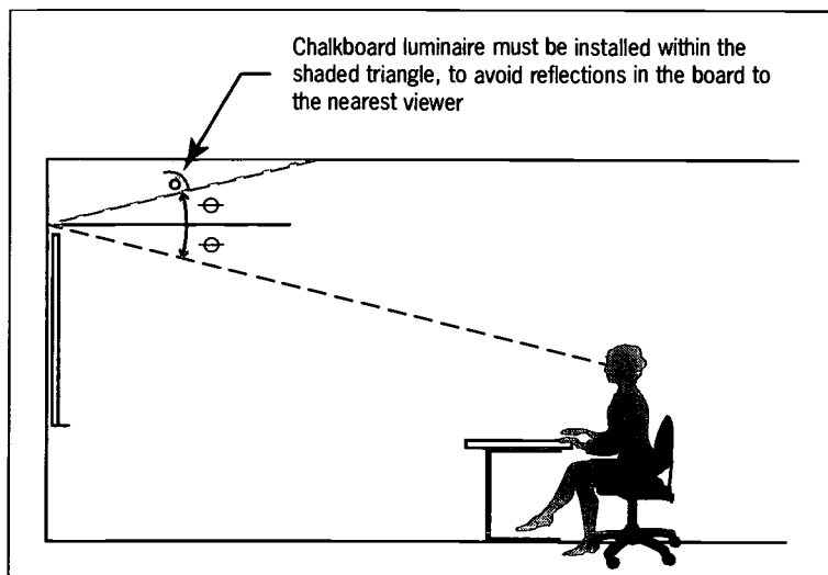
Figure 42: Chalkboard lighting
