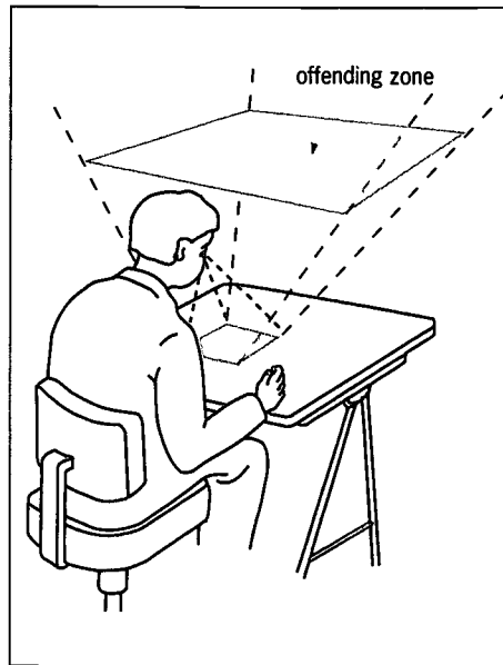
Figure 24: Veiling reflections, schematic diagram of 'offending zone'.
