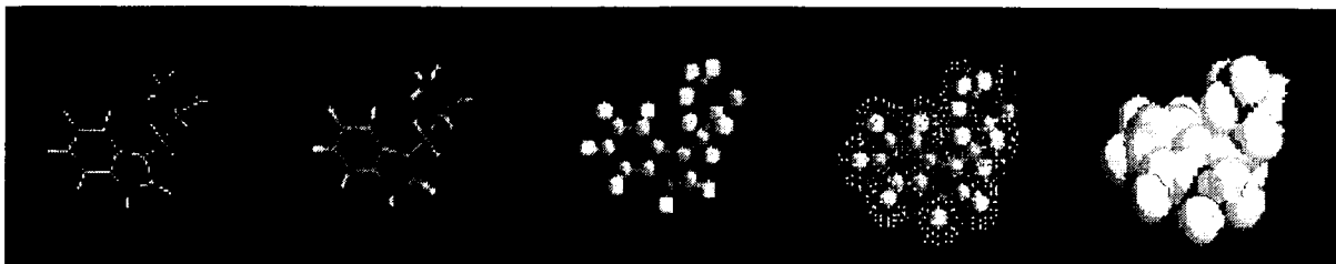
Figure 2: Chime Image Views of the Tryptophan Amino Acid Molecule
