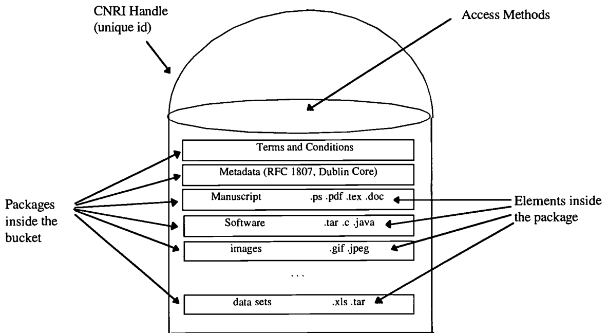
Figure 1: Bucket Architecture
