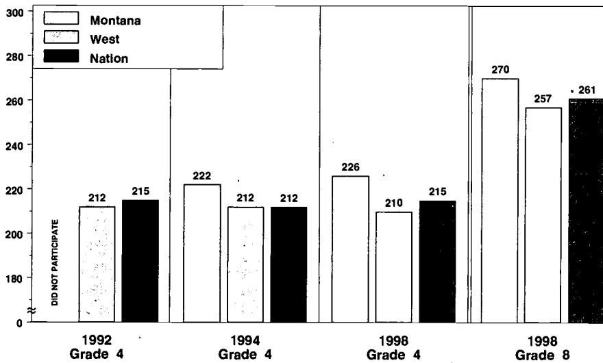
THE NATION'S REPORT CARD 1998 State Assessment FIGURE 1 Average reading scale scores for public school students at grades 4 and 8
