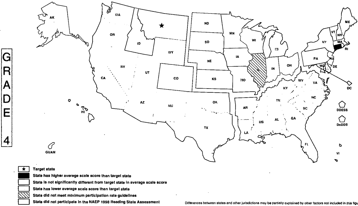
FIGURE 3 Montana's 1998 average reading scale score compared to those for other participating jurisdictions for public school students at grades 4 and 8
