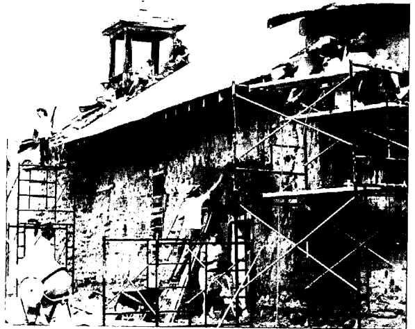
Members of the community of Ojo Caliente restoring their historic Santa Cruz Church (c.1790) with assistance from CORNERSTONES, Community Partnerships. The church is now fully restored. Photo by Steve Peart.
