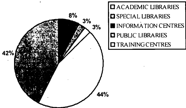
Graph 1. CDS/ISIS Users
