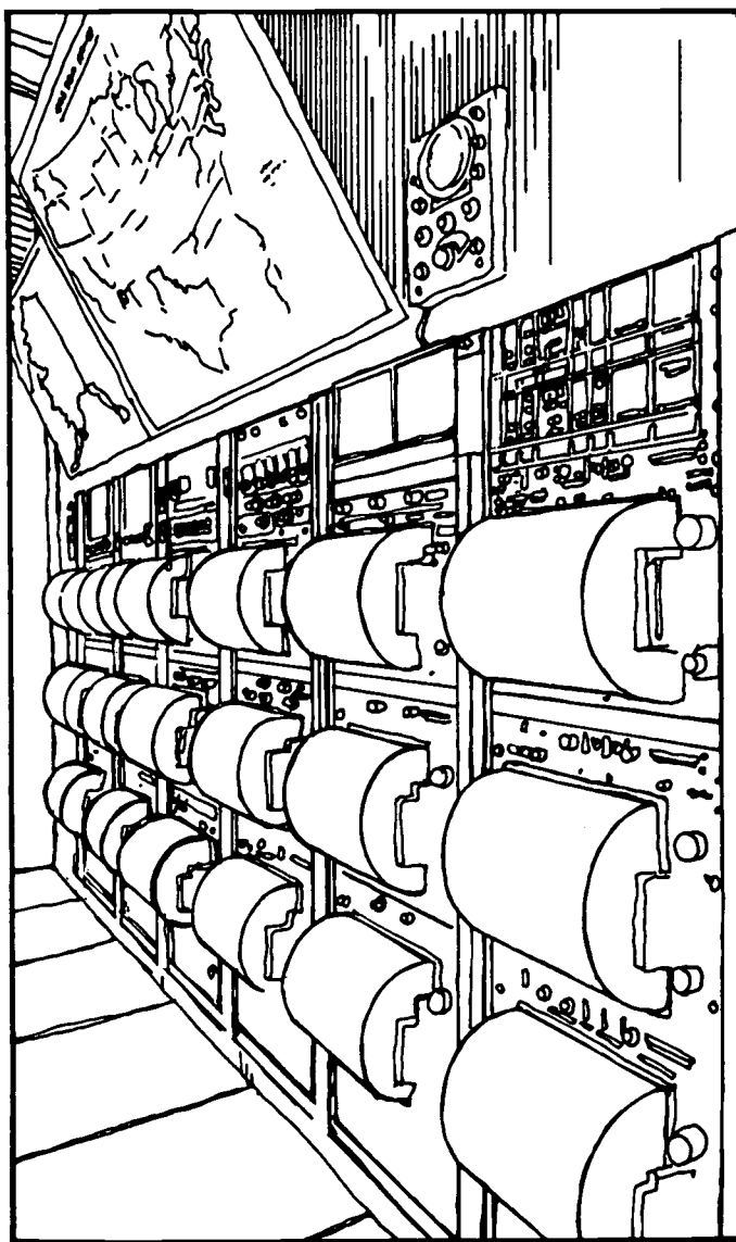
Modern seismographs
