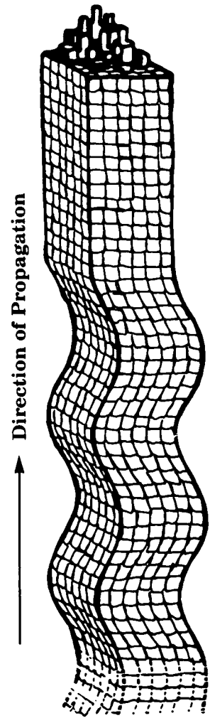
S Waves
