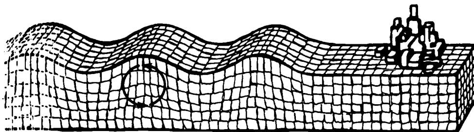
Rayleigh Waves
