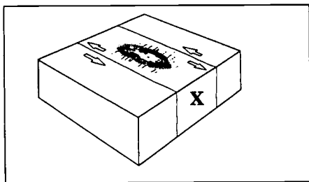
Right Lateral Strike-Slip Fault
