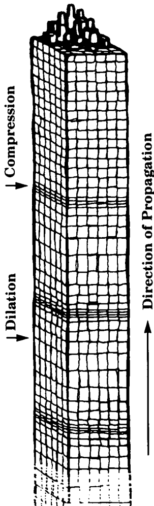
P Waves
