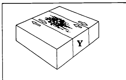
Left Lateral Strike-Slip Fault
