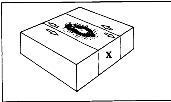
Right Lateral Strike-Slip Fault
