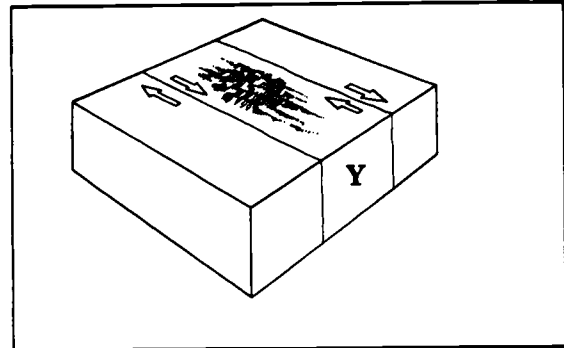
Left Lateral Strike-Slip Fault
