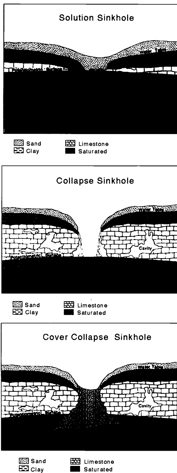
Figure 11.1: Three major types of sinkholes
