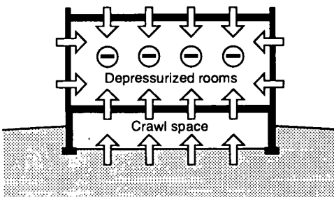
Figure 1-4: Some mechanical ventilation systems are not properly balanced resulting in depressurization of the interior spaces in a building. This can induce radon to enter spaces and must be addressed in a mitigation effort.
