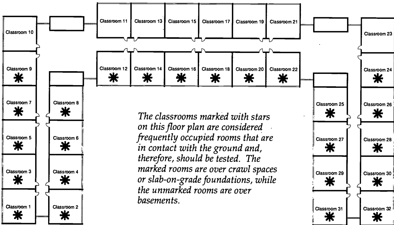
Figure 5-1: Floor plan of school.
