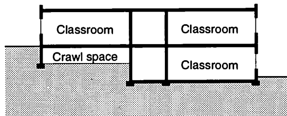
Figure 4-4: Cross section A-A' of part of a typical school.
