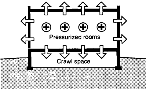
Figure 1-3: Mechanical ventilation can be designed to pressurize the interior spaces in a building by bringing in outdoor air. This may help reduce radon entry by pressurizing the building and diluting radon.
