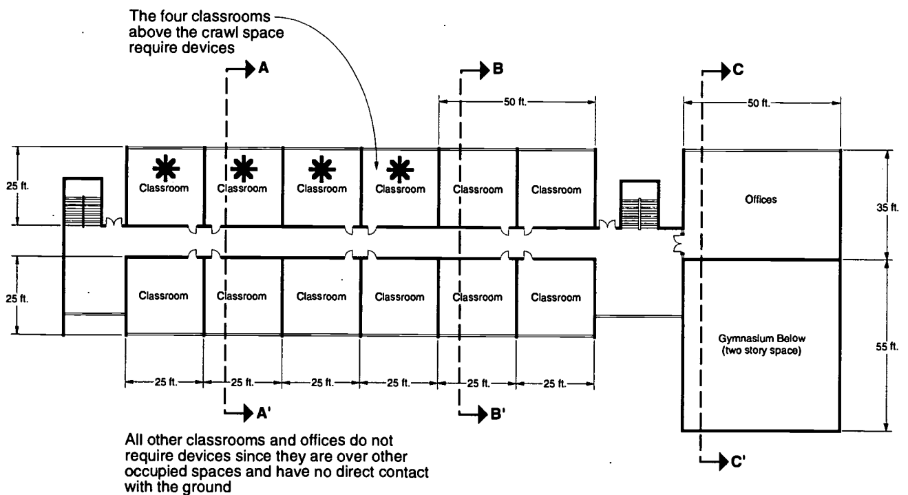
Correct answer for Figure 4-8: Upper level plan of a typical school showing placement of detectors.
