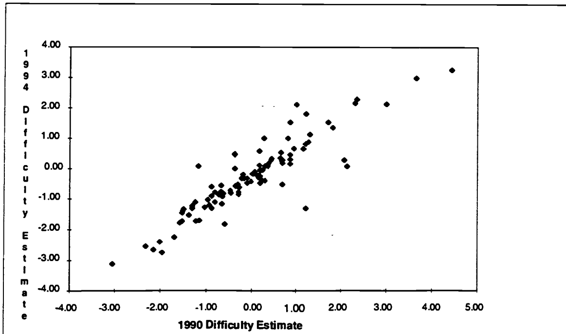
Figure 9-2: Comparison of Item Difficulty Parameter Estimates from the 1990 and 1994 Reading Long-Term Trend Assessments
