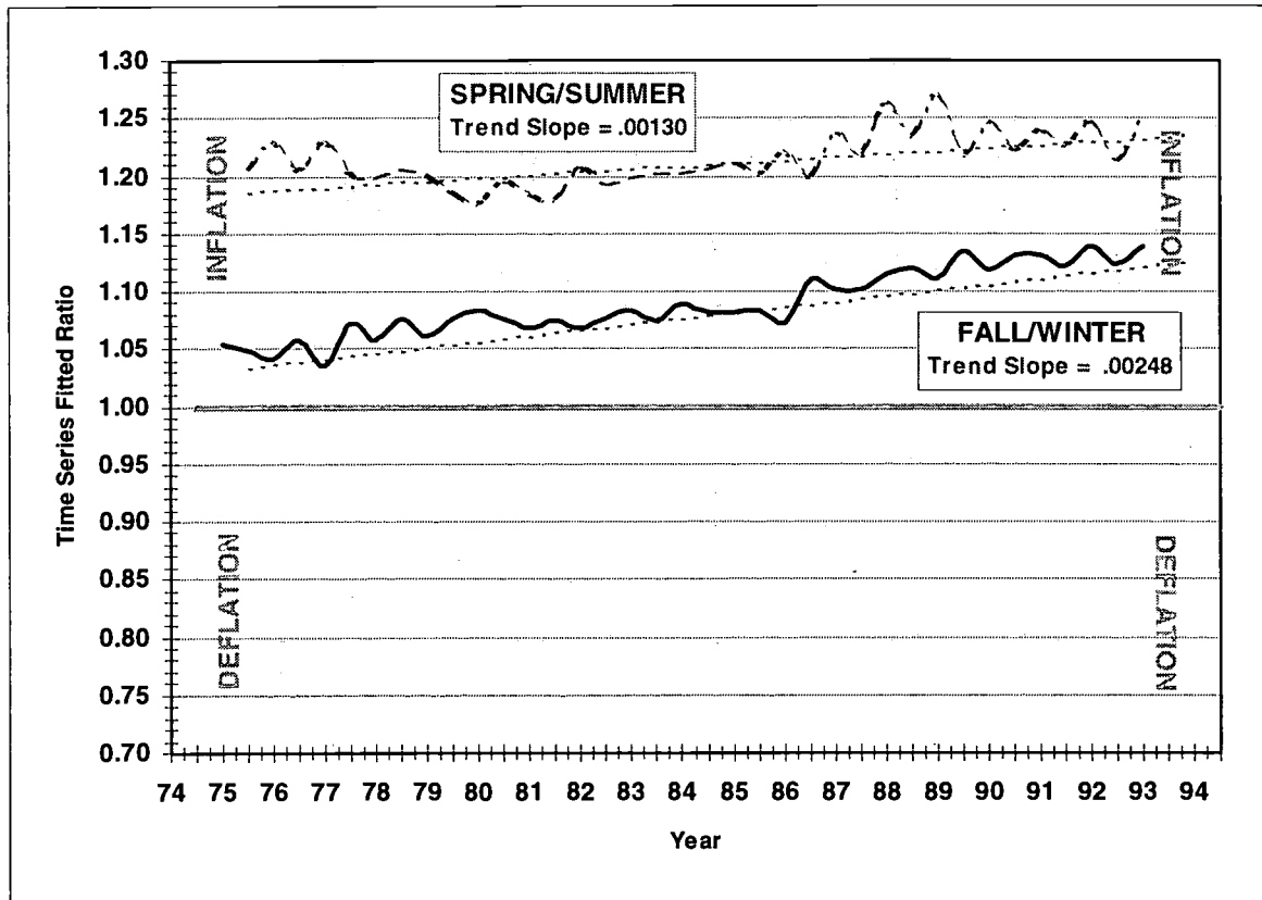
Figure 2. Fitted Ratios—College A
