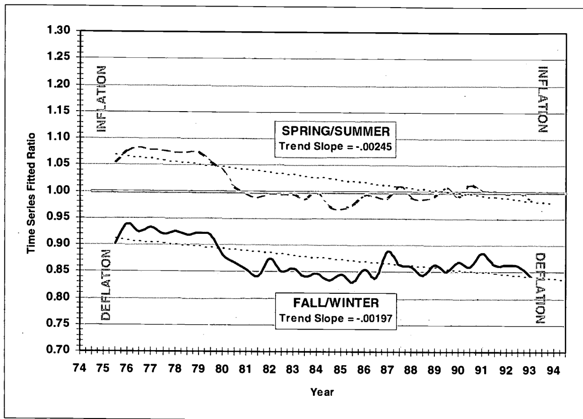
Figure 3. Fitted Ratios—College B
