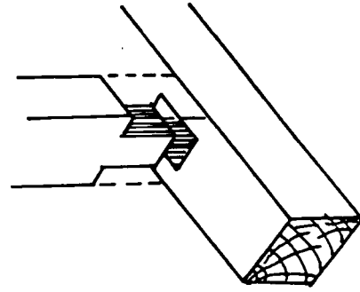
DOOR AND WINDOW FRAME JOINT DETAILS
