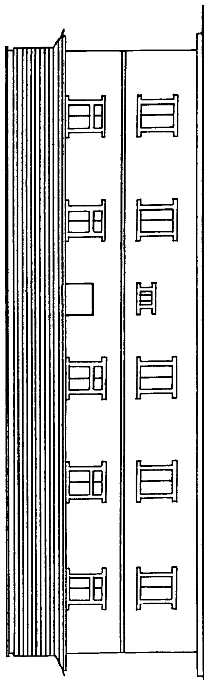
REAR ELEVATION
