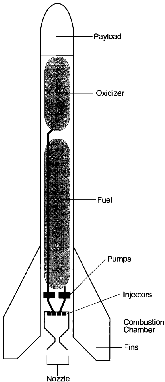
Liquid Propellant Rocket
