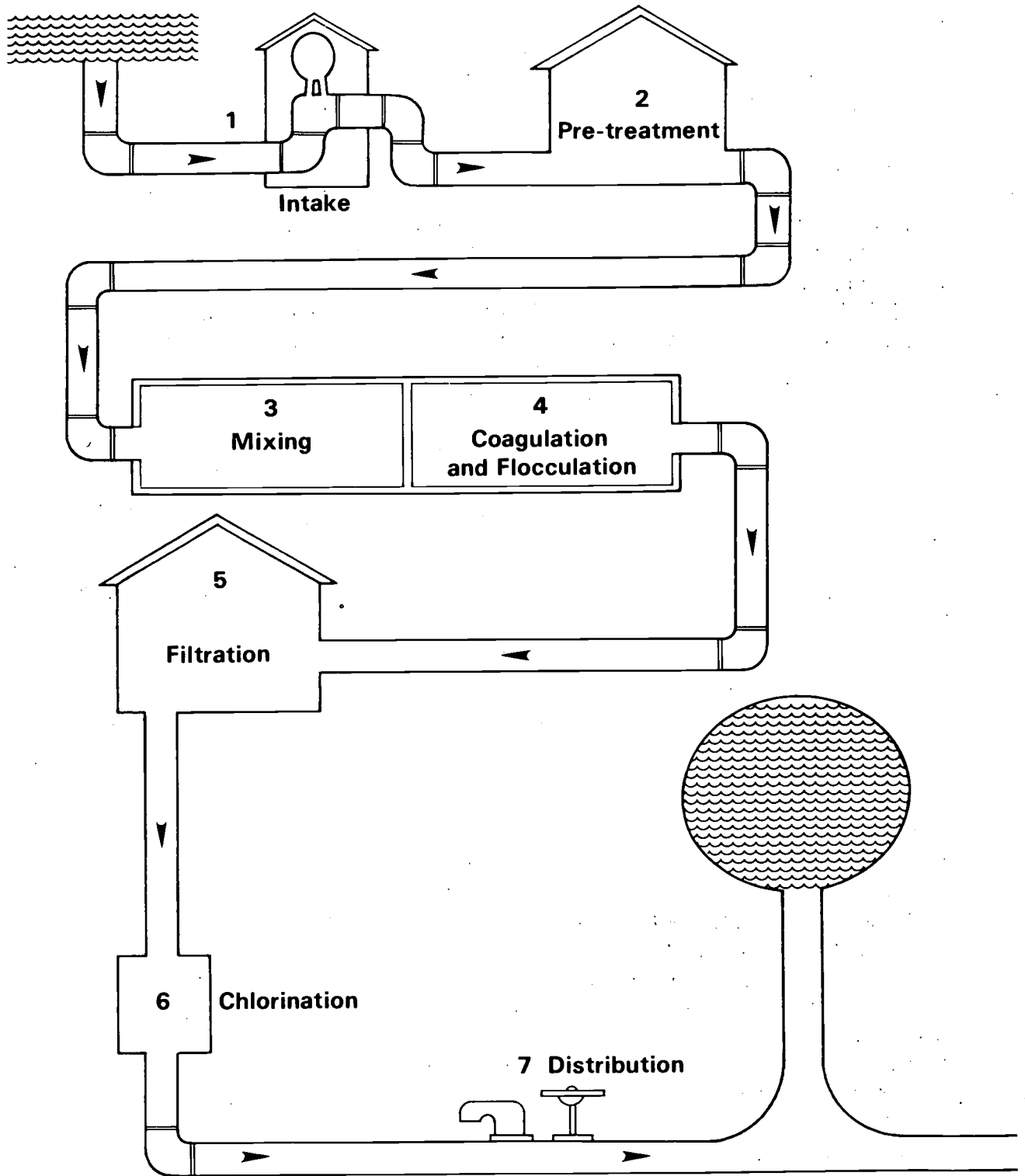
The Drinking Water Treatment Process
