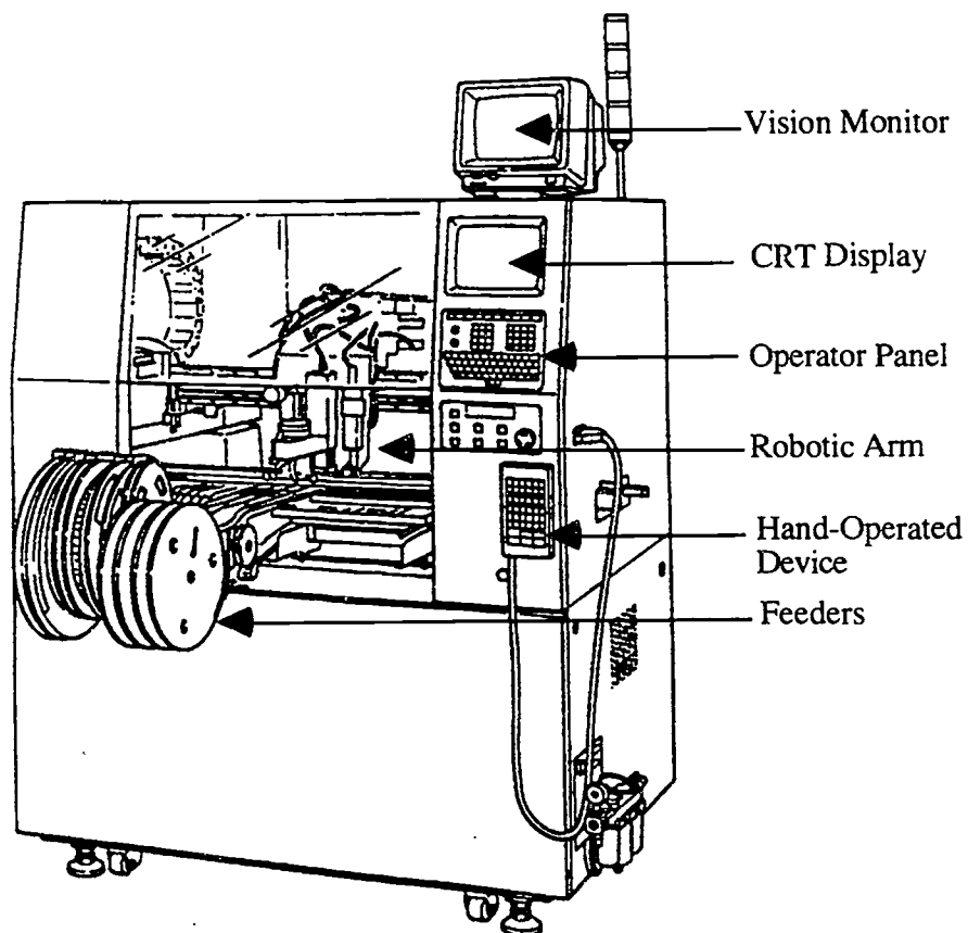
Figure 1 SMT Machine
