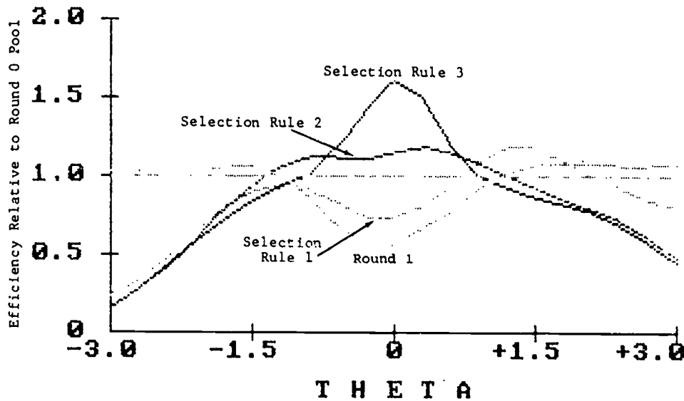
Figure 10. For Elimination Rule 2: Estimated test information functions for the 100-item pools resulting from each Selection Rule of the current study, the Round 1 pool of the previous study, and for the Round 0 pool (top); efficiency of each 100-item pool relative to the Round 0 pool (bottom).
