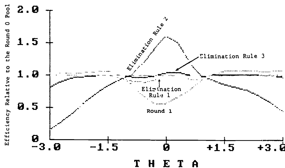
Figure 8. For Selection Rule 3: Estimated test information functions for the 100-item pools resulting from each Elimination Rule of the current study, the Round 1 pool of the previous study, and for the Round 0 pool (top); efficiency of each 100-item pool relative to the Round 0 pool (bottom).
