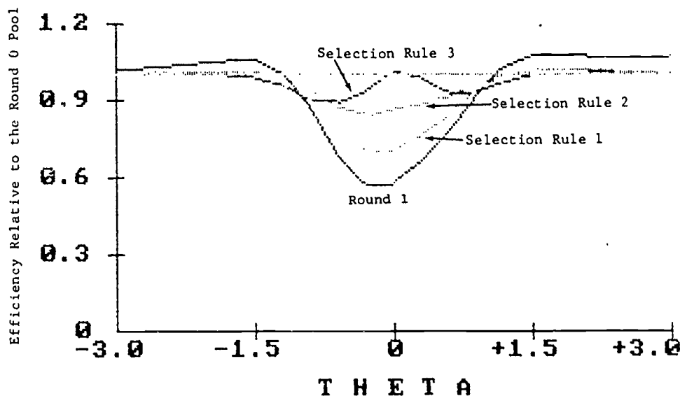
Figure 9. For Elimination Rule 1: Estimated test information functions for the 100-item pools resulting from each Selection Rule of the current study, the Round 1 pool rule of the previous study, and for the Round 0 pool (top); efficiency of each 100-item pool relative to the Round 0 pool (bottom).
