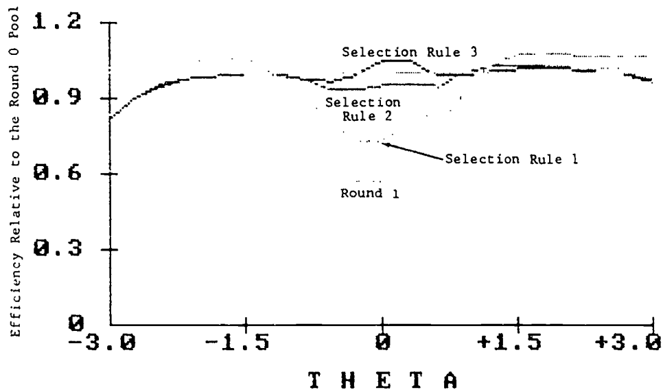
Figure 11. For Elimination Rule 3: Estimated test information functions for the 100-item pools resulting from each Selection Rule of the current study, the Round 1 pool of the previous study, and for the Round 0 pool (top); efficiency of each 100-item pool relative to the Round 0 pool (bottom).
