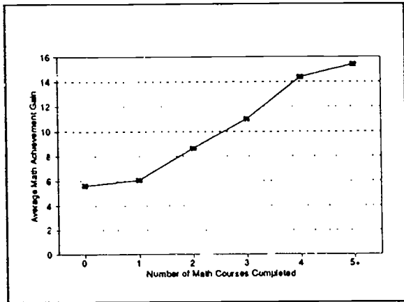
Figure 2.-- Average mathematics test score gain from 8th- to 12th-grade, by number of mathematics courses completed during high school: 1992
