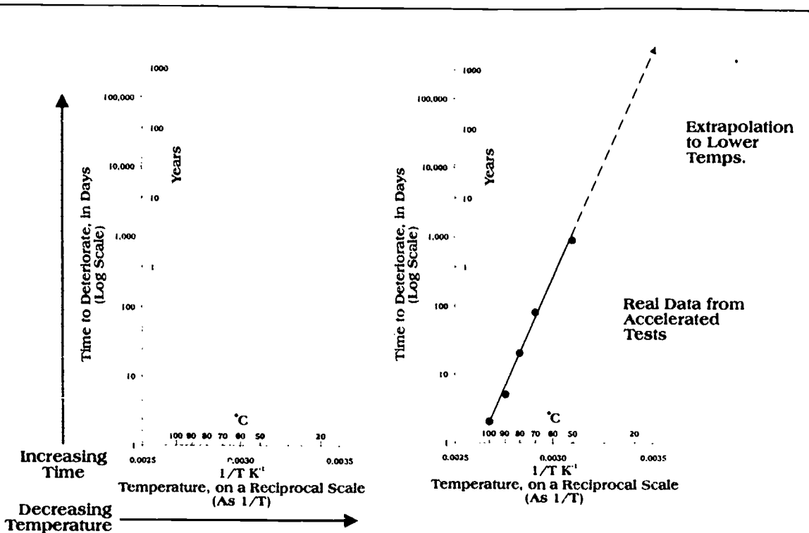
Figure 11. Sample Arrhenius plot, axes only.
