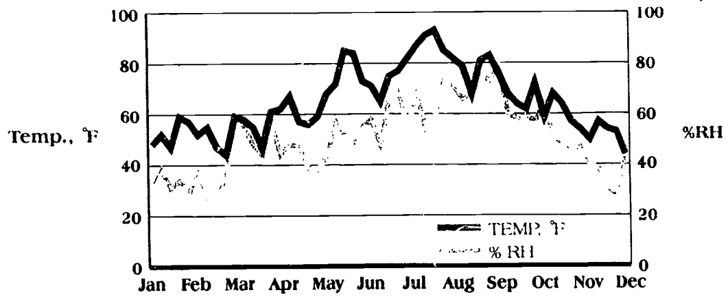
Figure 2. Attic temperature and RH.
