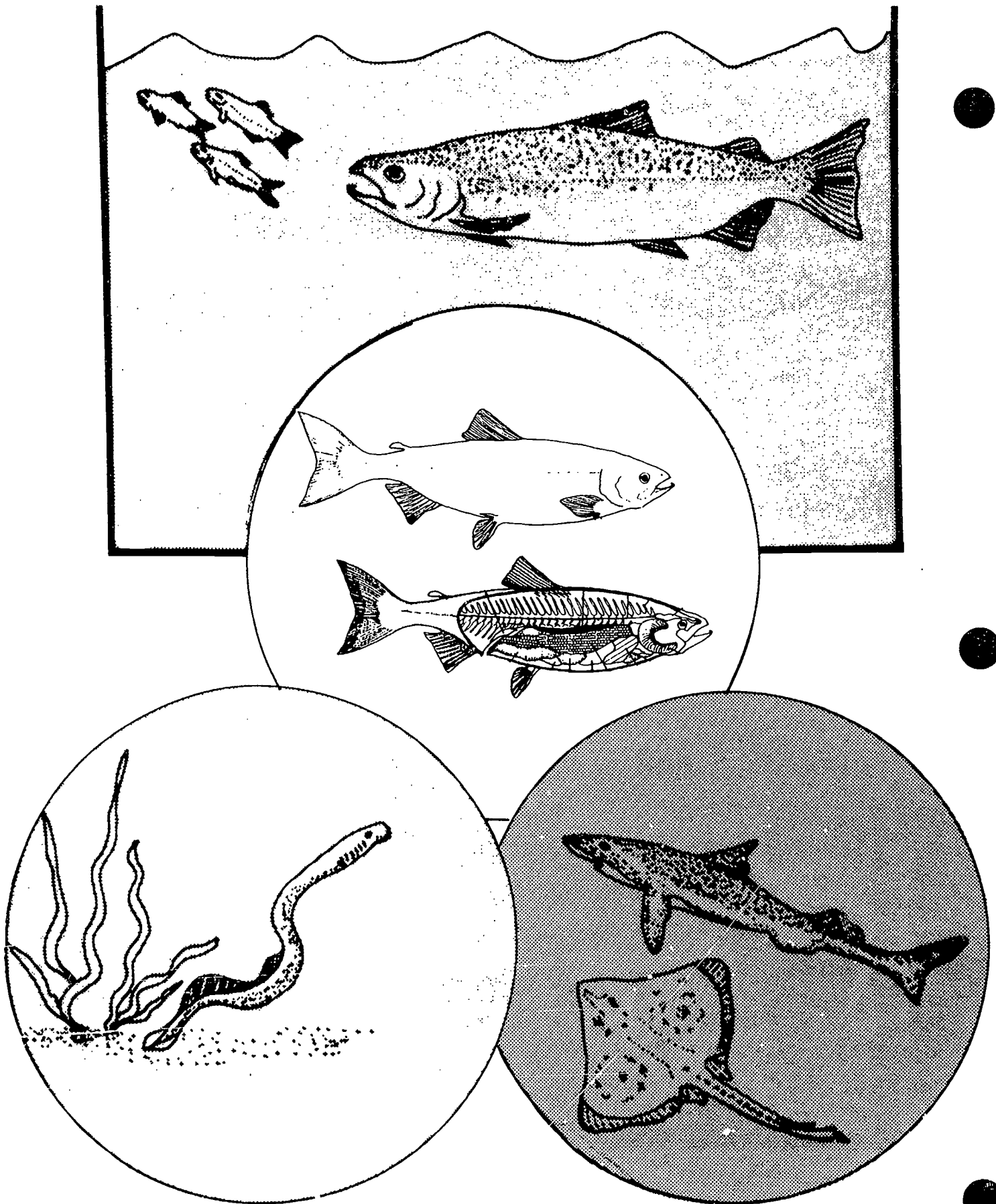
Unit One: The three major fish groups: bony fish (represented by salmon, top and center); hagfish and lampreys (represented by lamprey, lower left); and sharks, skates and rays.
