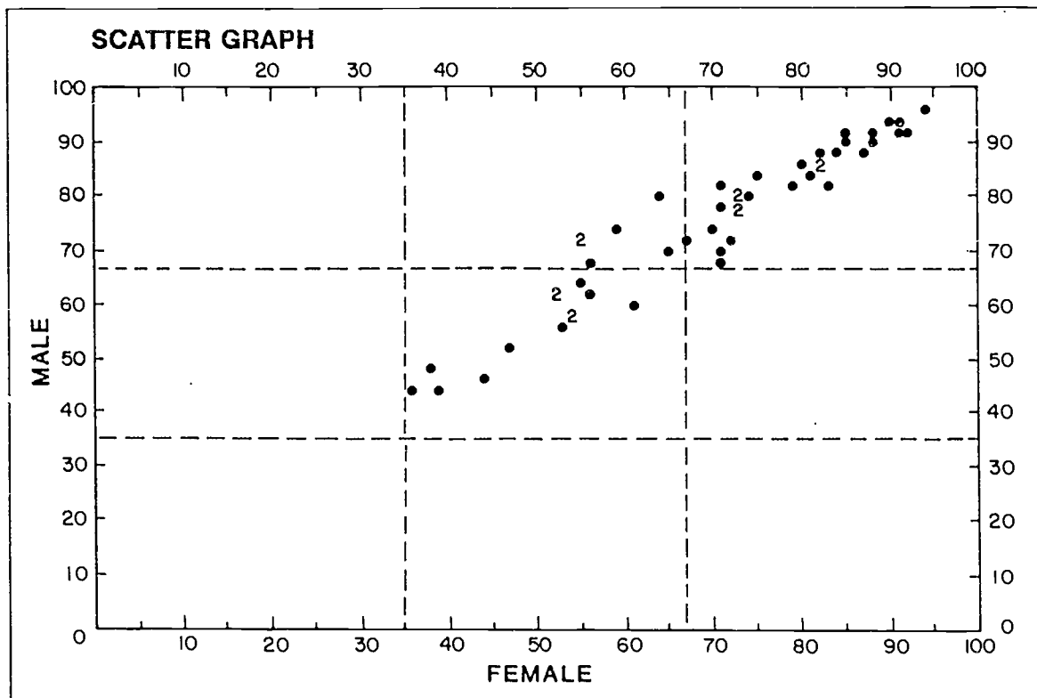
Figure 2. Example of a scatter graph of item difficulties comparing the performance of males with that of females.
