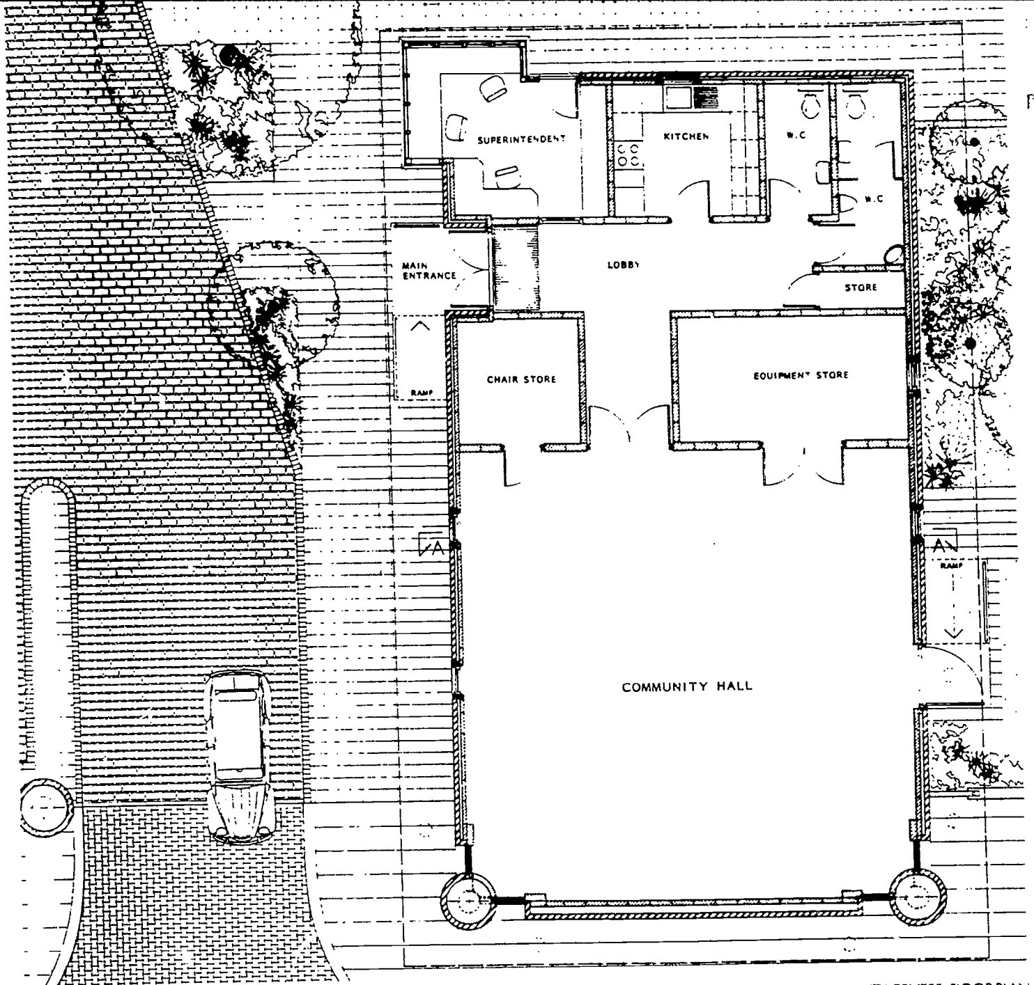
COMMUNITY CENTRE: FLOOR PLAN
