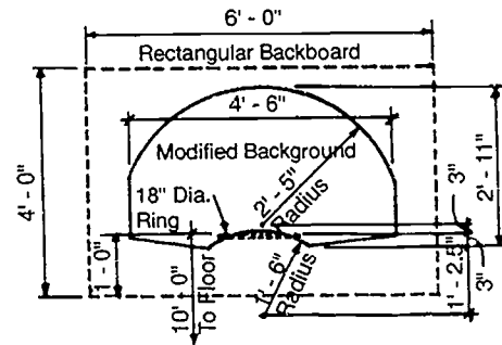
Backboard Detail
