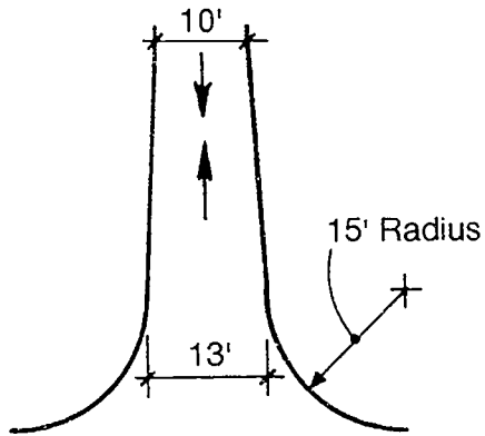
One Way Single Lane Entrance - Exit
