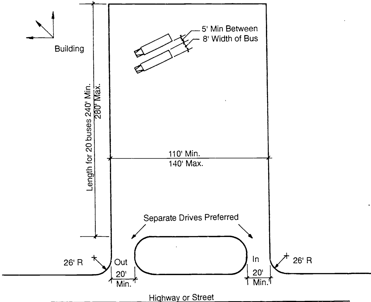
Bus Parking Layout
