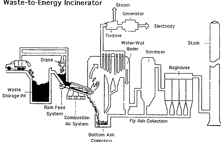
Typical Mass Burn Waste-to-Energy Incinerator
