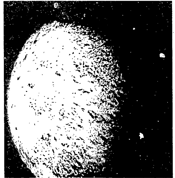
Neptune, currently the outermost planet in the solar system, and its largest satellite, Triton, were imaged close-up by NASA's Voyager 2 spacecraft in August 1989. Four times Earth's diameter but 30 times Earth's distance from the sun, Neptune is invisible to the naked eye. It was not even discovered until 1846 and appears little larger than the resolution limit of even the largest ground-based telescopes. Space missions such as Voyager involve large numbers of scientists, engineers, and mathematicians (NASA photographs)
