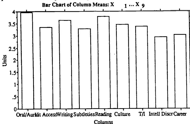
Graph 22a: Mean responses to questions 24 part 1 ...24 part 9
