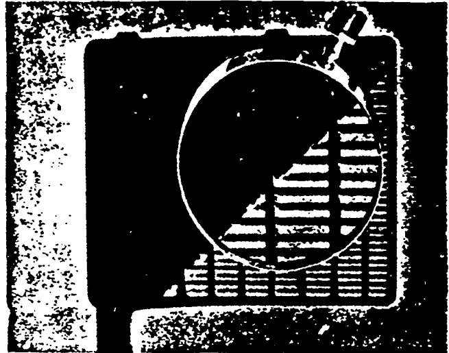
Fig. 3 Positive Plate With Part of Active Material Removed to Show Grid Structure.
