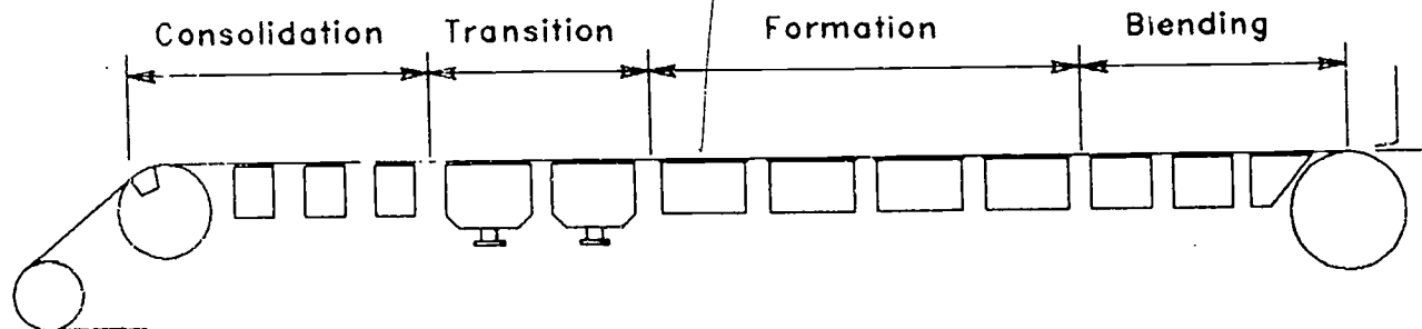
Figure 4-2. Example of Fourdrinier Drainage Zones
