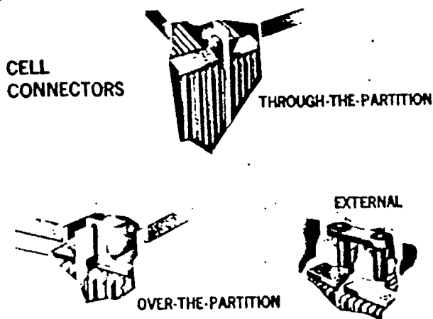
Fig. 7 Cell Connectors
