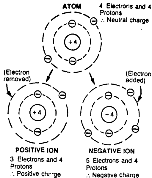
FIG.2 HOW ATOMS FORM IONS ( ibid , p.22)
