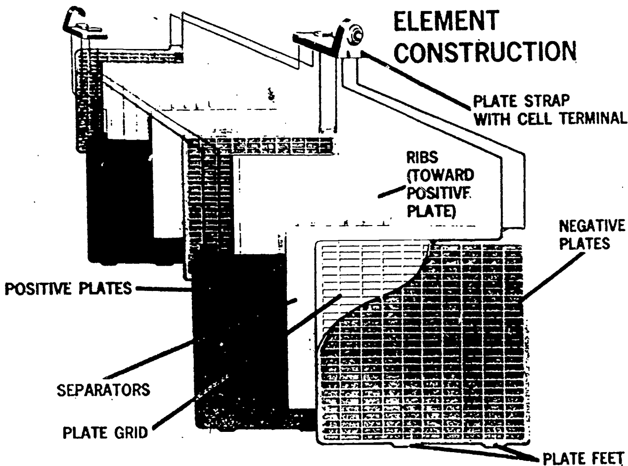
Fig. 4 Element Construction-Conventional Battery
