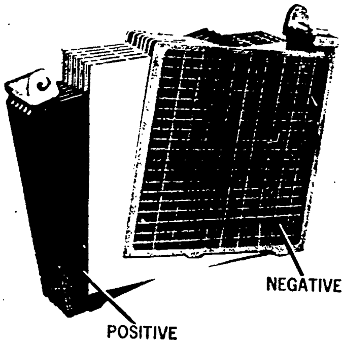
Fig. 5 Battery Element
