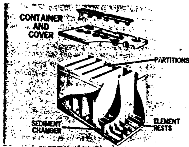
Fig. 6 Container And Cover-Typical
