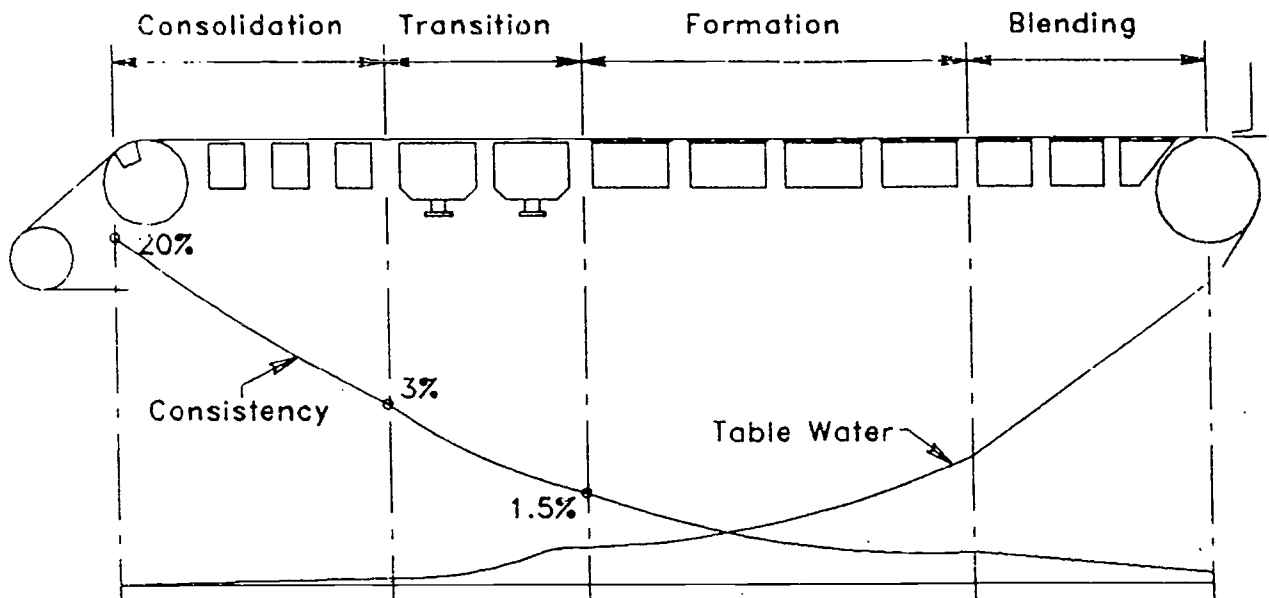
Figure 4-3. Fourdrinier Drainage Model
