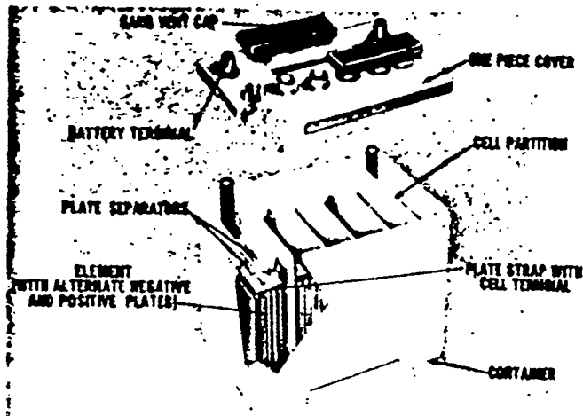
Fig. 9 The Complete Assembly-Conventional
