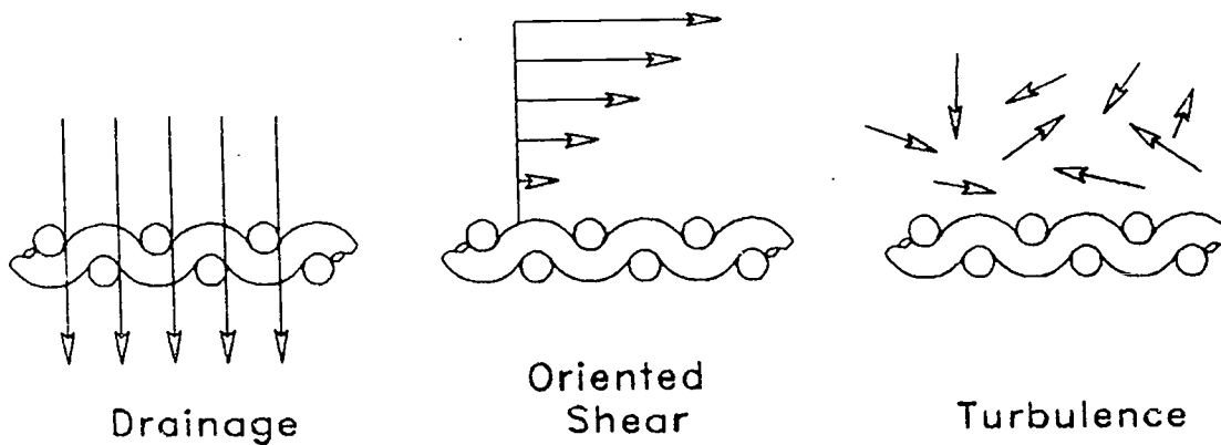
Figure 4-1. Forming Forces
