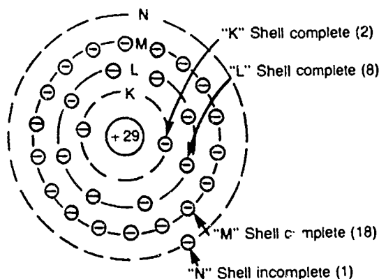
FIG.1 THE COPPER ATOM
