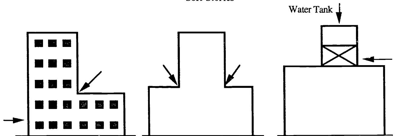
Sides of buildings where the upper stories are not as big as the lower stories Setbacks
