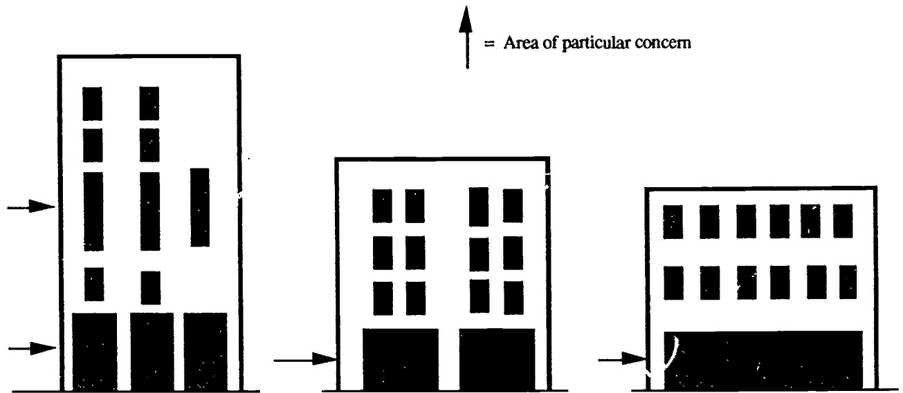
Sides of buildings - Solid walls are above shorter walls or columns Soft Stories
