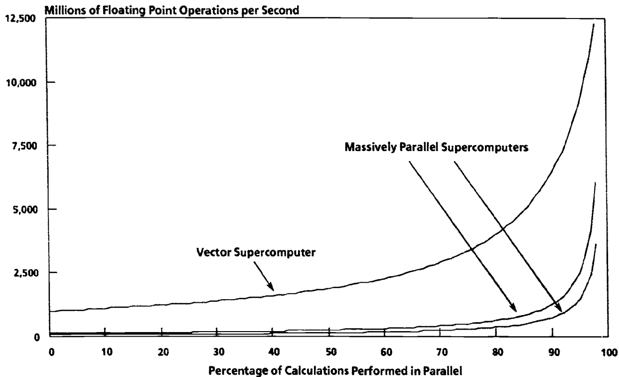
Figure 3. Simulated Performance of Three Supercomputers
