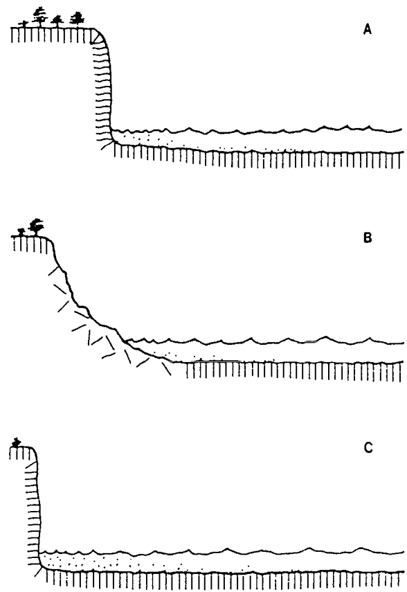
Figure 5.6. The erosional cycle. (A) Erosion at the slope toe during high lake level. (B) Slope failure. (C) Erosion of the debris deposited by slope failure and renewed erosion at the slope toe.
