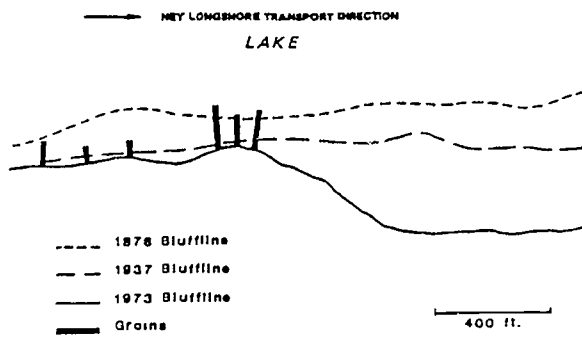
Figure 5.8. Accelerated erosion at Painesville-on-the-Lake east of the Fairport Harbor jetties. Local erosion caused by groins is greatly amplified by sand trapped at Fairport Harbor.
