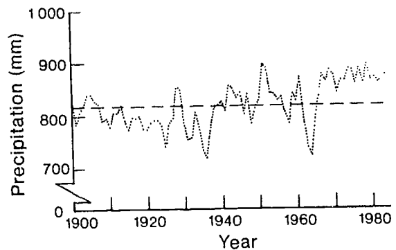
Figure 11.3. Historic precipitation.
