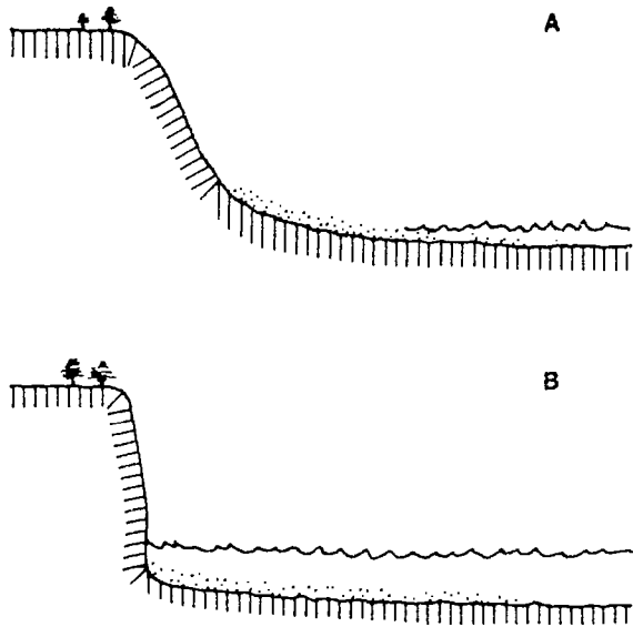
Figure 5.4. Effect of lake level on wave erosion. Wave energy lost to the beach at a low lake level (A), and wave energy expended on the shore at a high lake level (B).
