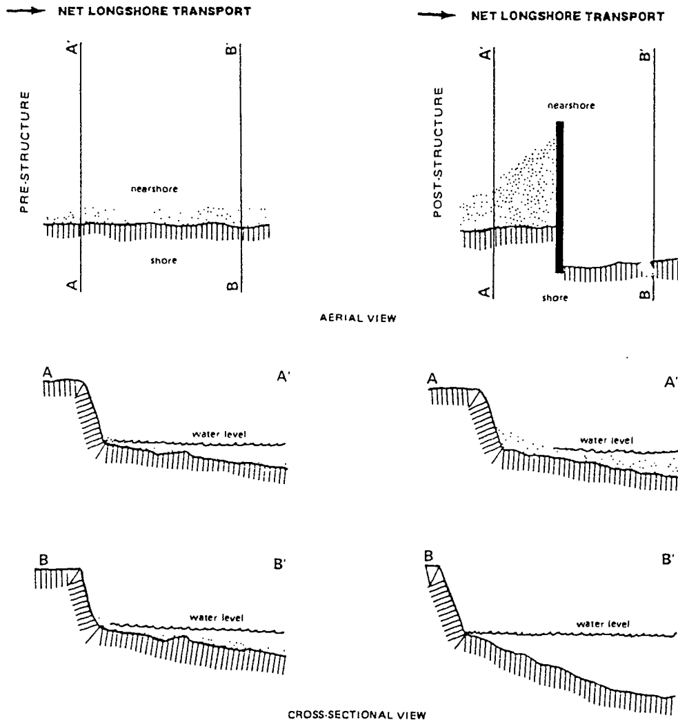
Figure 5.9. Changes caused by a groin. (from Carter and Guy, Ohio Geological Survey Report Inv. 115)
