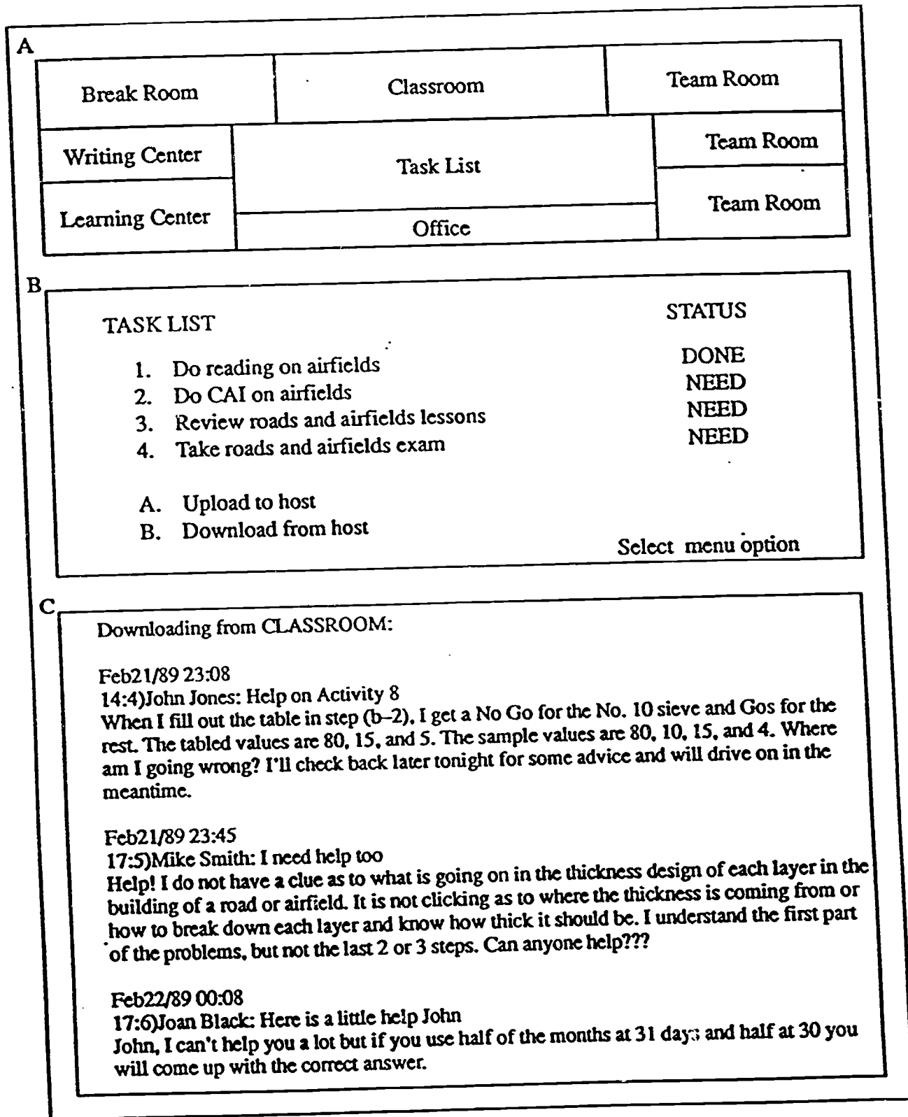
Figure 4. Sample SMART session.
