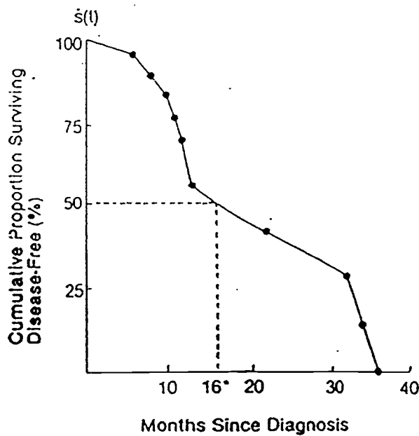
FIGURE I SURVIVAL ANALYSIS
