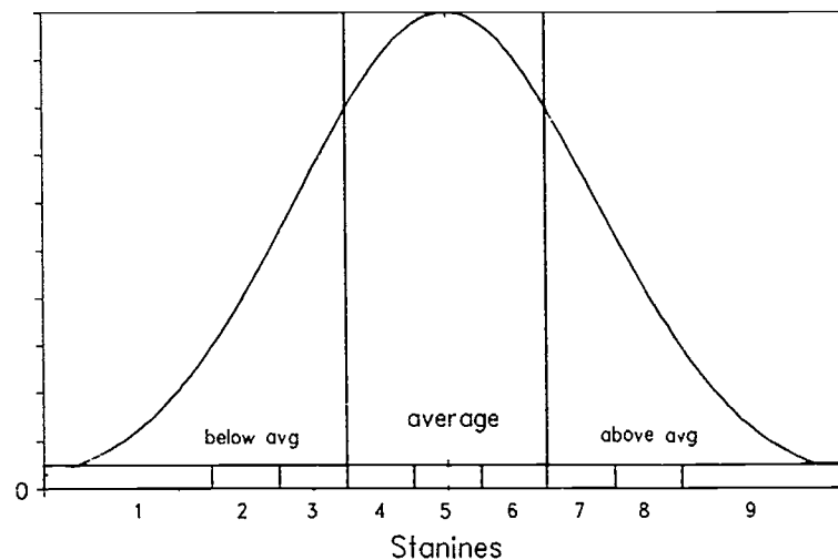
Stanines and the Normal Curve
