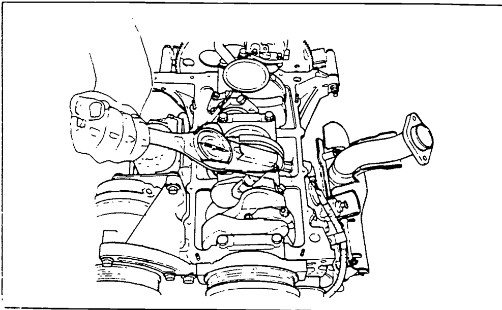
Applying Correct Torque to Rod Bearings
