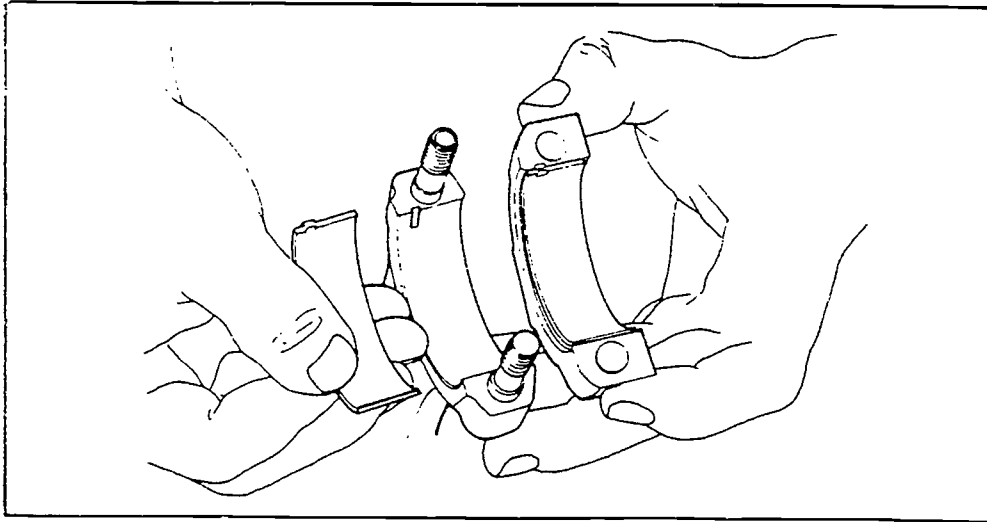
Installing Connecting Rod Bearings
