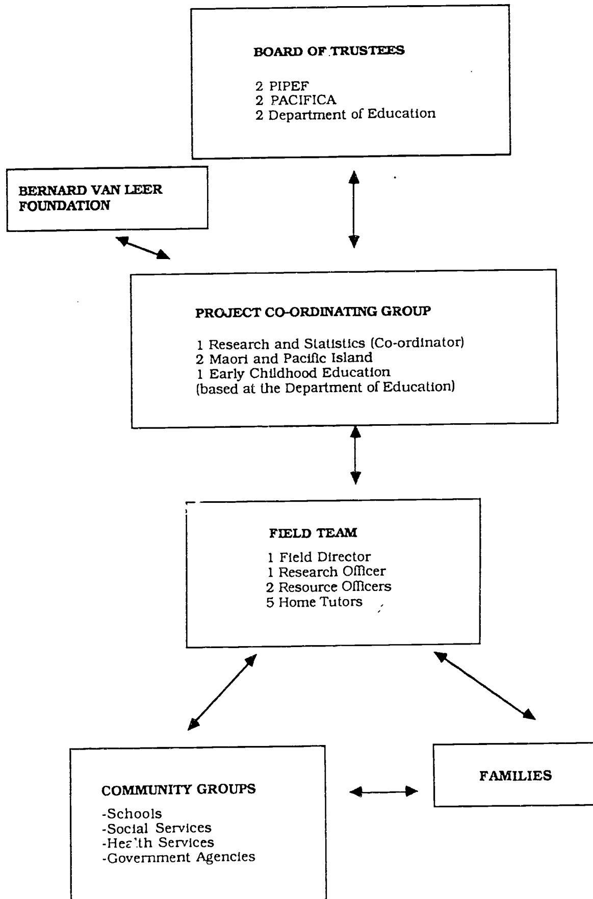
Figure 1. Project Organisation
