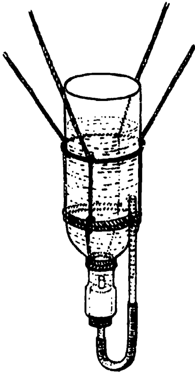
Barometer
