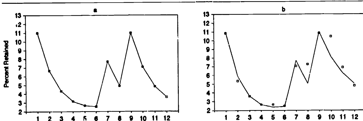
Figure 1 The exponential model of retention rates, as an ideal function (graph a), and as fitted to the median values of 12 American states (graph 1b). The "ideal" pattern shown in Figure 1a is expressed mathematically as r = k + c(1-p)^x , where r ("the r function") is the retention rate and x indicates time in period, in school-years. The k , c , and p are positive constants that represent the minimum rate, the initial rate (peak) less the minimum, and the inclination of the curve, respectively, and p never exceeds unity. The horizontal axis represents grades 1 through 12. The square symbols connected by the line mark the value of the function at that point. The square symbols in 1b represent the medians of 12 states for the year 1979-80; and the line represents the function as fitted to them. The graphs in this figure are reproduced from Morris (1990).
