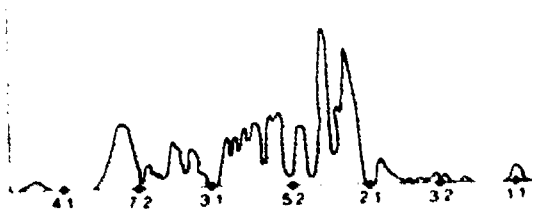
FIGURE 10. Gaps and clumps in the distribution of asteroids reveal resonance with the orbital period of Jupiter.
