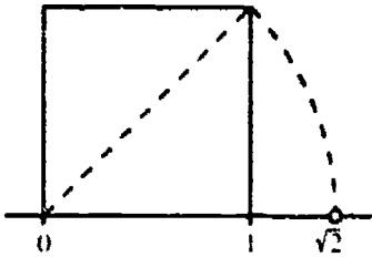
FIGURE 8. The position on a rational number line corresponding to the length of the hypotenuse of a right triangle with legs of length 1 has a hole, since there is no rational number equal to \sqrt{2} .
