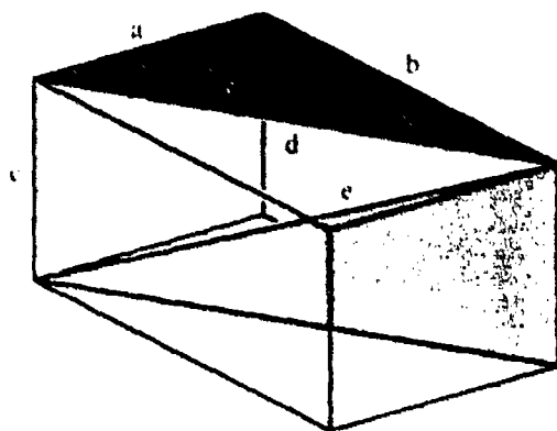
FIGURE 32. Generalizing the Pythagorean theorem to three dimensions by applying it to two different triangles found in a rectangular box.
