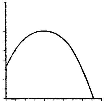
FIGURE 3. The standard parabolic trajectory becomes visible in a graph of the height of a projectile as a function of its time in flight.
