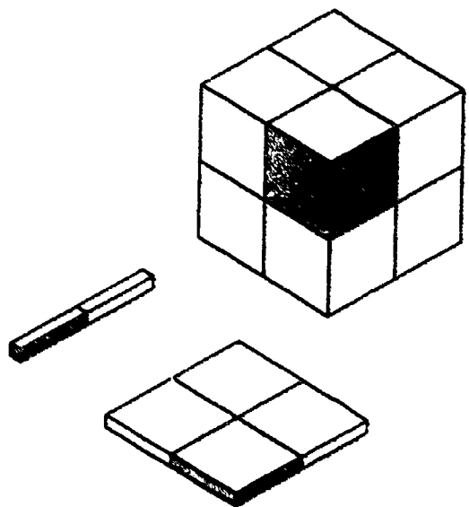
FIGURE 17. Nested cubes, squares, and rods illustrate the fundamental property of doubling factors: they represent the power of 2, depending on dimension.
