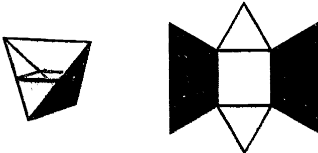
FIGURE 38. As the central slice of a six-sided cube yields a regular six-sided polygon, so the central slice of a four-sided tetrahedron yields a regular four-sided polygon—that is, a square. The template on the right provides the means for constructing half of a tetrahedron; two such pieces make an excellent geometric puzzle.
