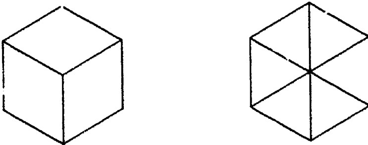
FIGURE 23. The symmetric "isometric" view of a cube, both solid and transparent, arise by looking at one corner at a 45^\circ angle. Then the opposite corner lies directly behind the front corner, so only seven vertices are distinguished in this view.
