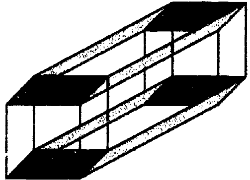
FIGURE 44. Shading helps identify two horizontal groups of four parallel squares in the hypercube. There are six such groups in all, three associated with the original cube and its displaced copy and three associated with the edges that join the two cubes.
