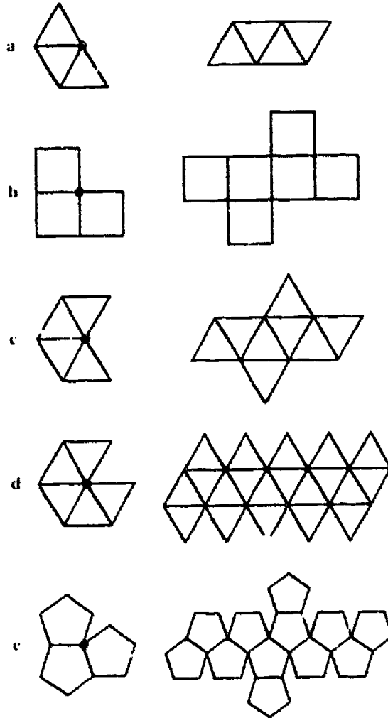
FIGURE 2. There are only five regular polyhedra because there are only five arrangements of congruent, regular polygons about a point that can be folded up to make a convex polyhedral vertex. Here we see the five arrangements, together with their completion as patterns that can be folded up to make the entire polyhedron.
