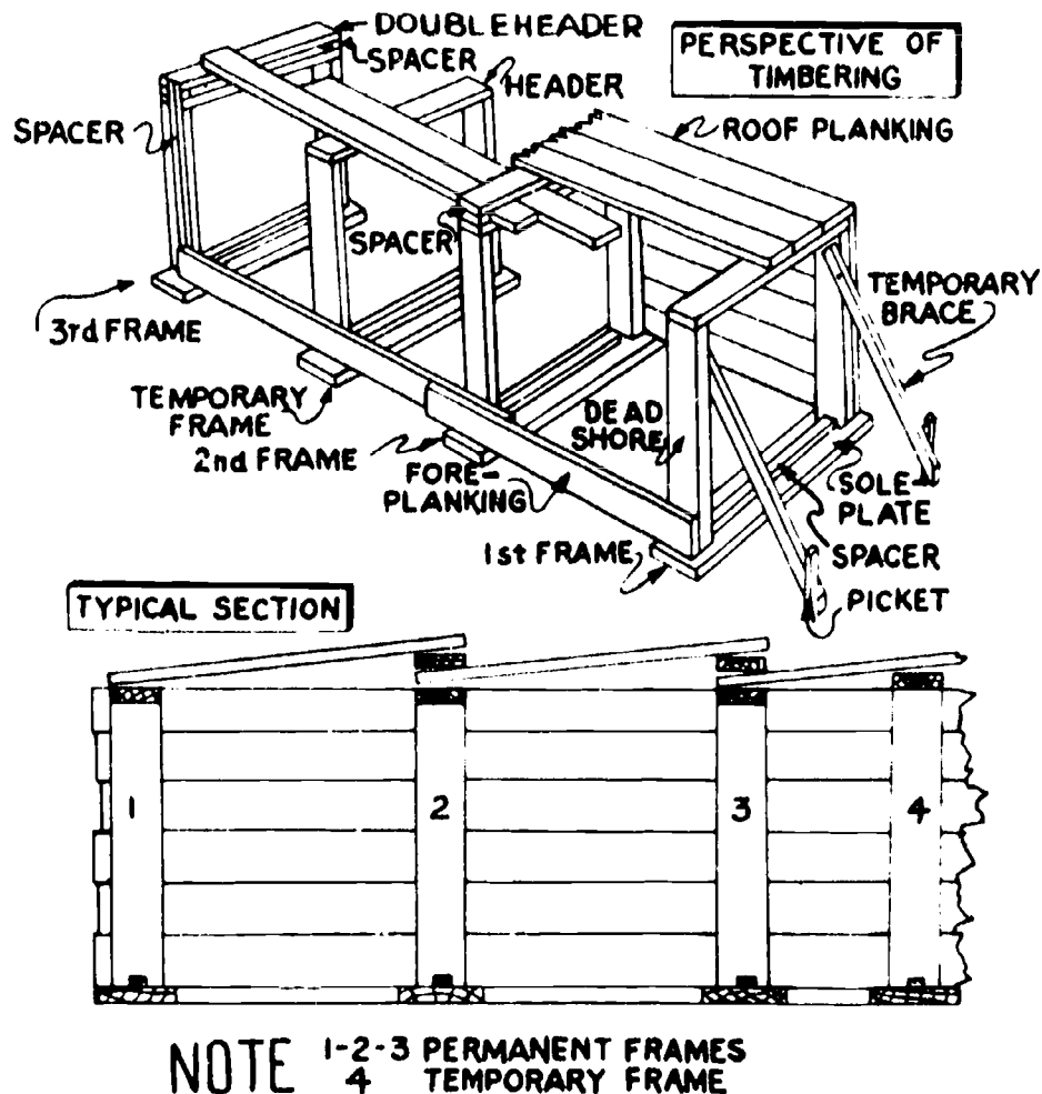
Figure 14. Tunnel Construction Using the Forepole Method
