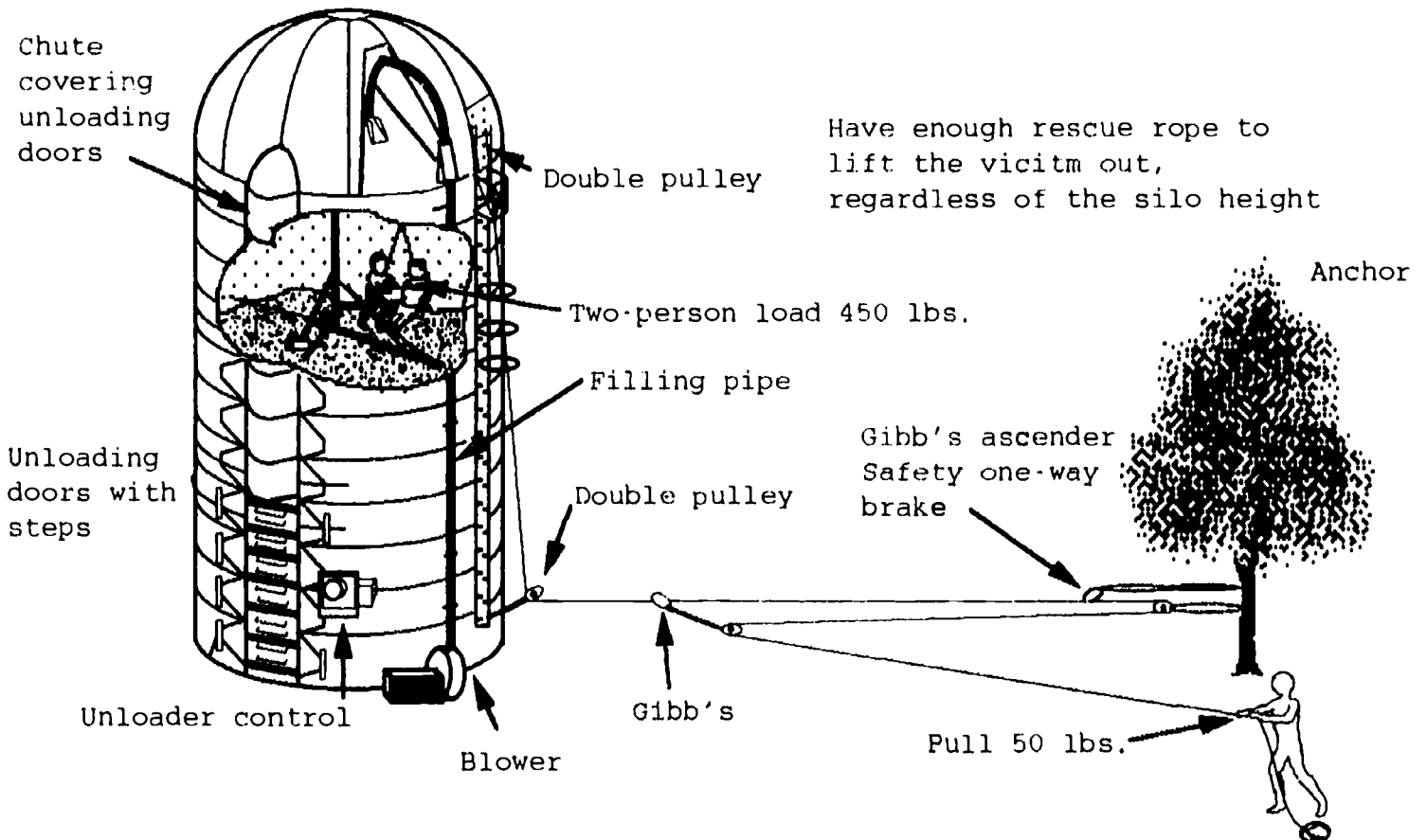
Figure 53. Hauling System, "Z" Drag
