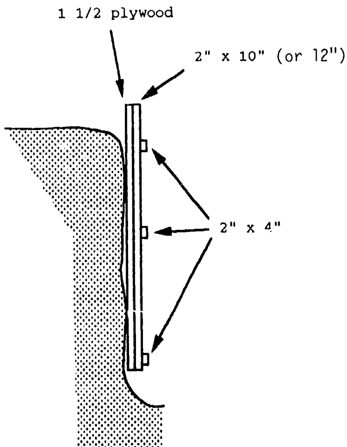
Figure 4. Shoring Against a Wall
