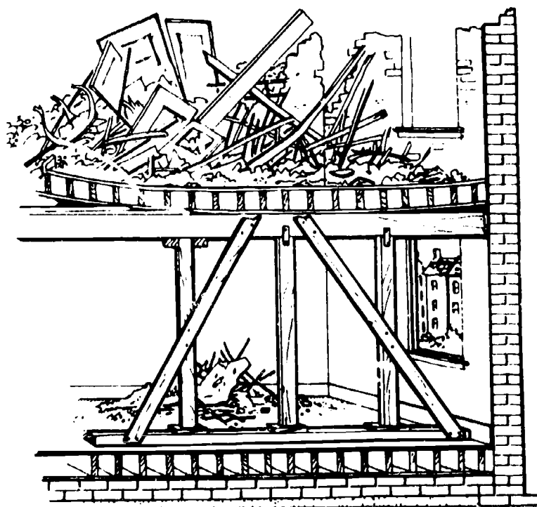
Figure 23. Dead or Vertical Shore
