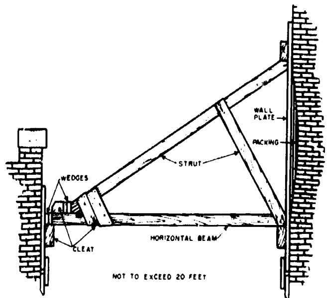
Figure 22. Flying Shores
