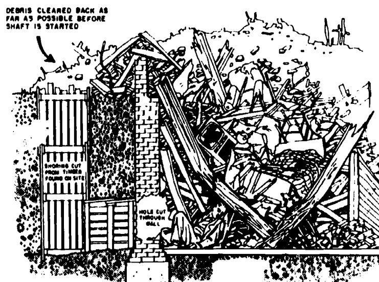
Figure 13. Shafting and Tunneling to Reach a Void
