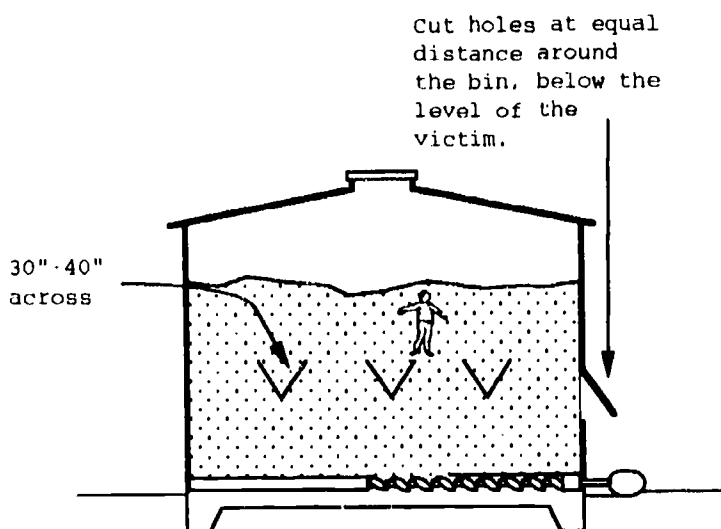
Figure 44. Releasing Grain from Bottom of a Bin
