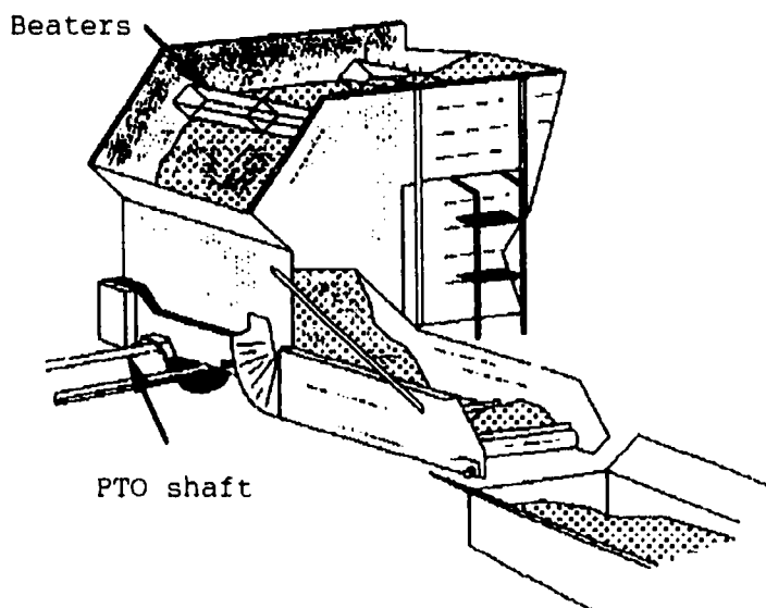
Figure 33. Self-unloading Wagon
