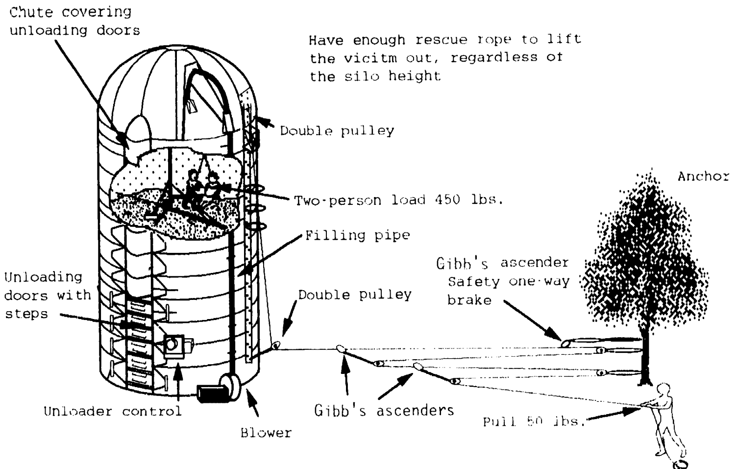
Figure 54. Hauling System, Stacked "Z" Drag
