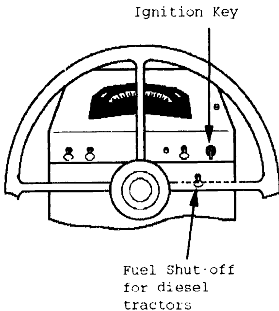
Figure 27. Tractor Panel
