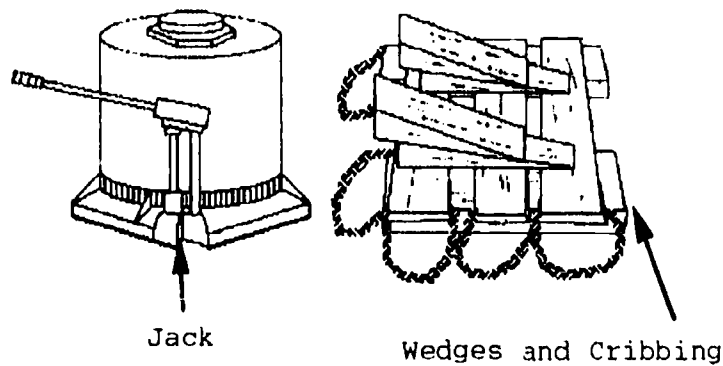
Figure 29. Cribbing, Wedges, and Jack
