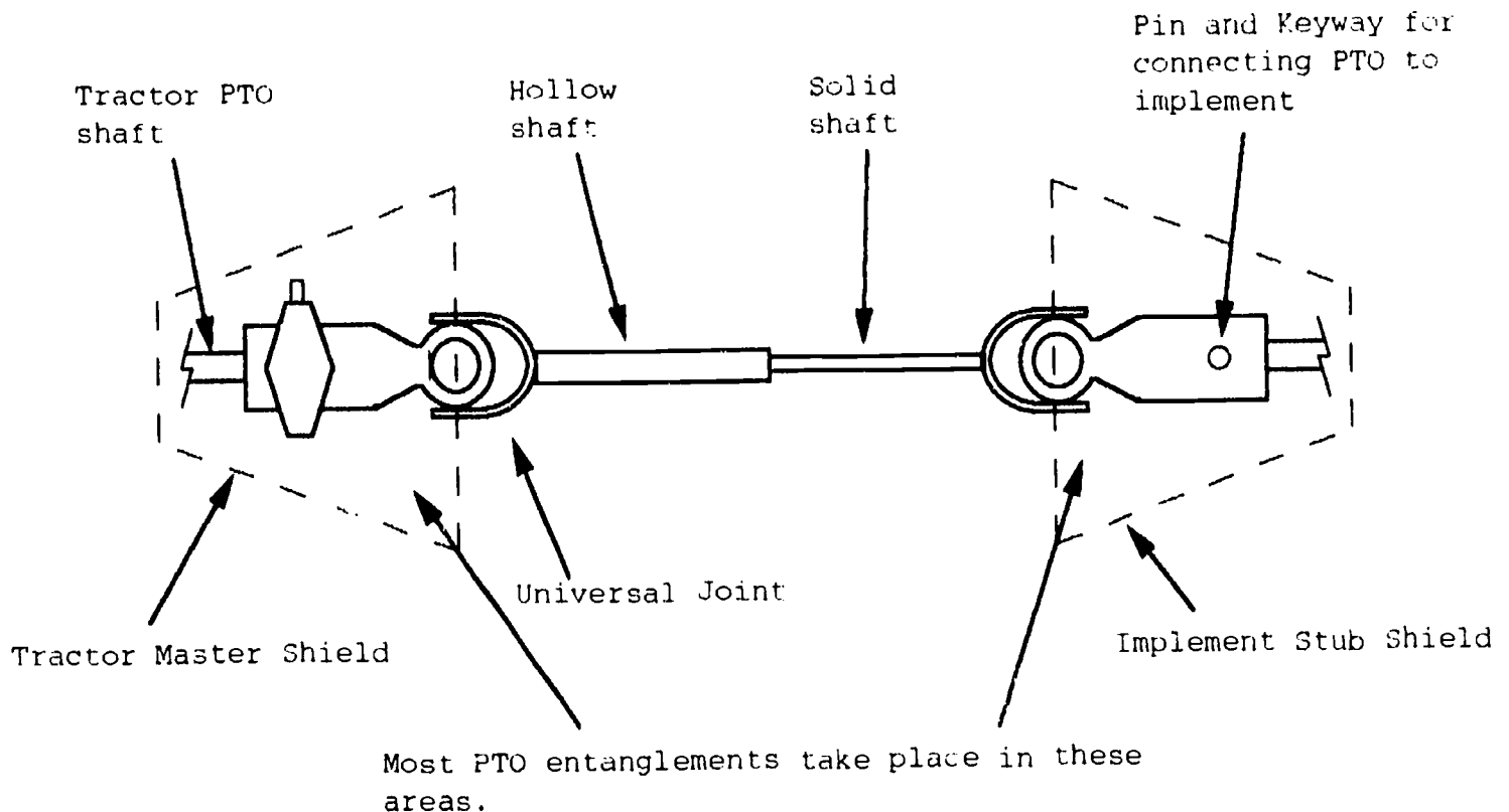
Figure 31. Power Take-off Shaft Diagram
