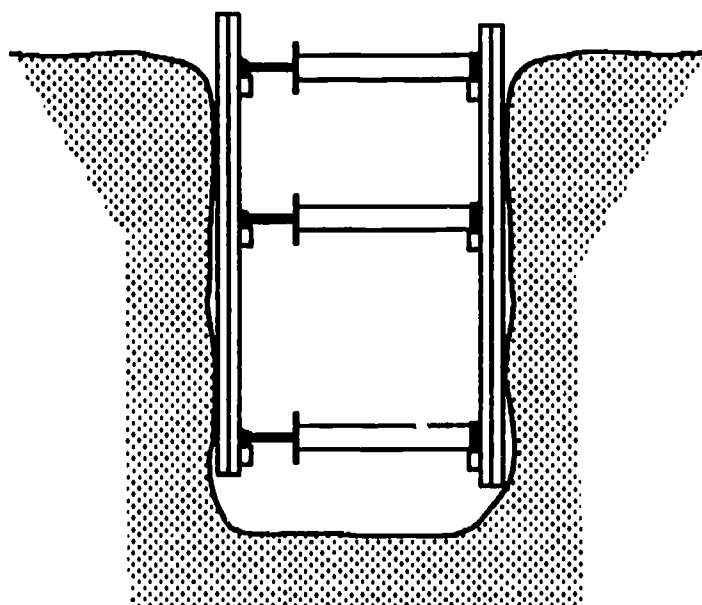
Figure 5. Supporting Jacks
