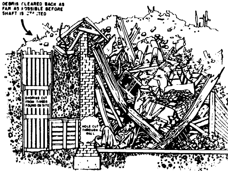
Figure 18. Shafting and Tunneling to Reach a Void
