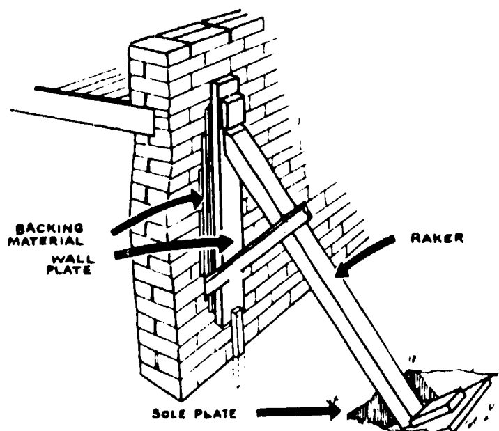
Figure 20. Raking Shore
