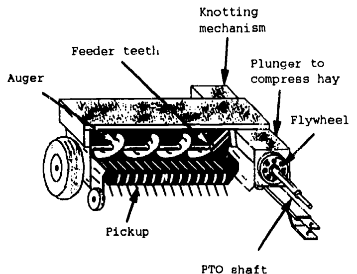
Figure 39. Conventional Baler
