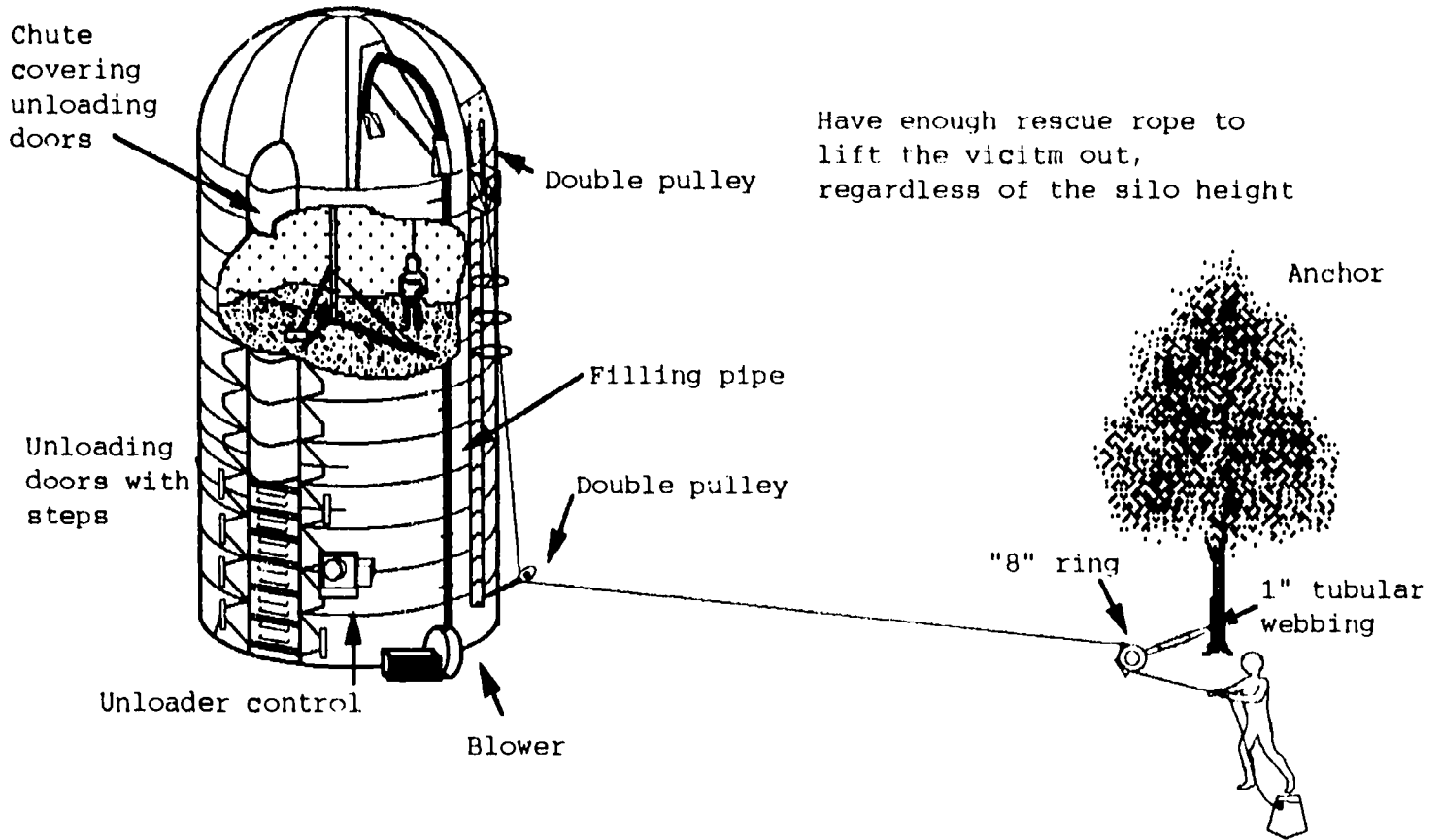
Figure 52. Lowering and Belaying System
