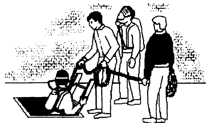
Figure 59. Entering a Manure Storage Facility
