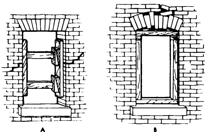
Figure 24. Strutting a Window Opening
