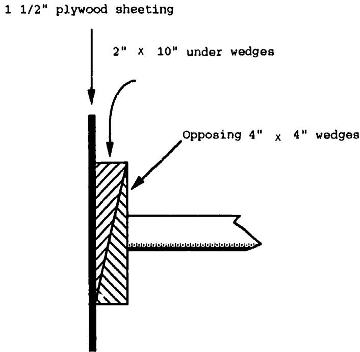
Figure 6. Wedges Used to Support Shoring
