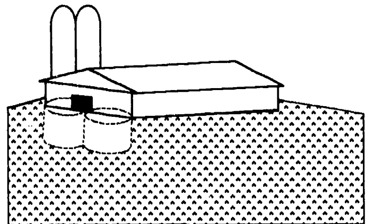
Figure 58. Below Ground Manure Storage
