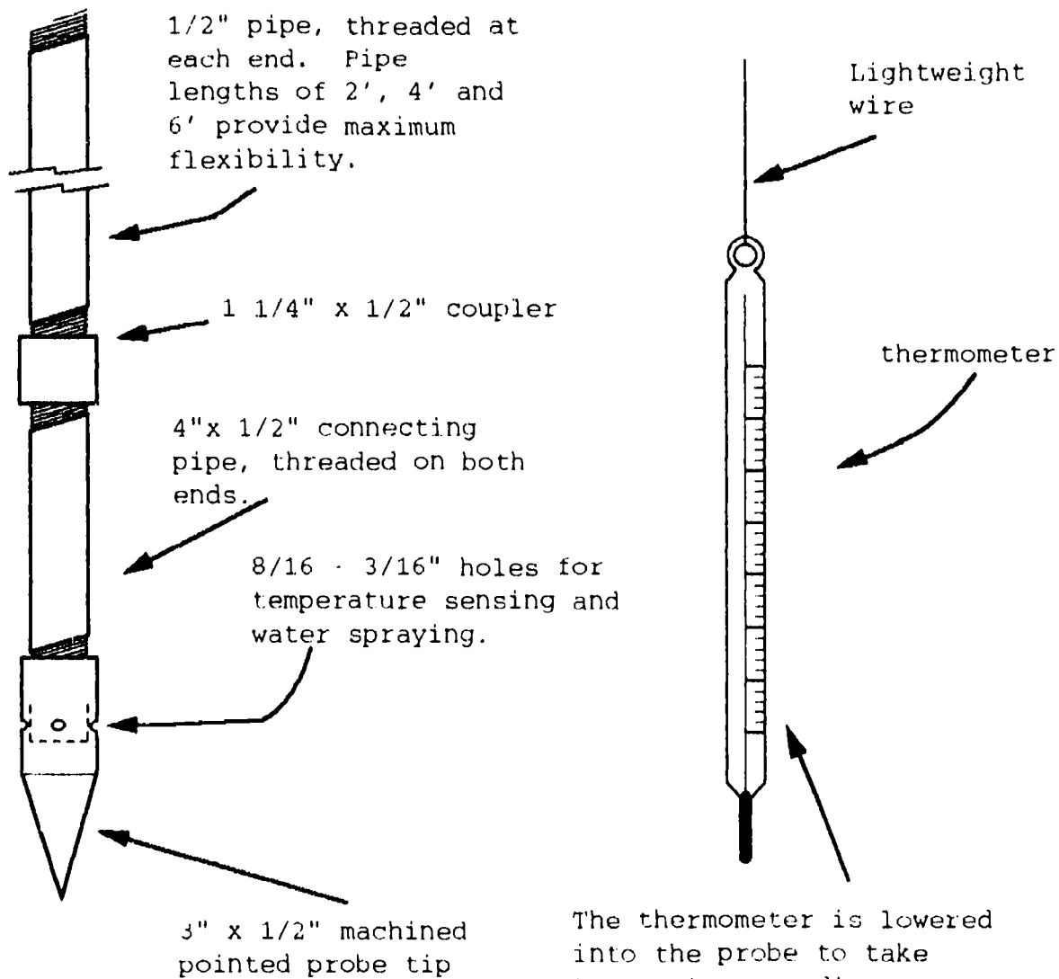
Figure 55. Probe and Thermometer
