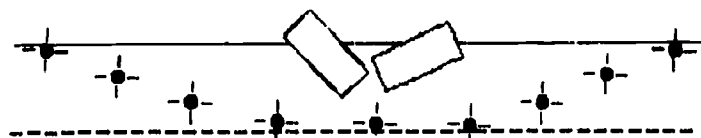
Figure 69-A. Display of warning devices on a straight section of road
