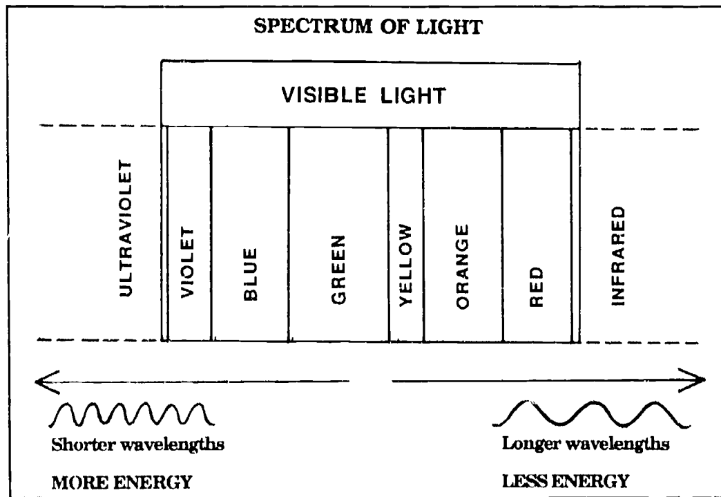
Figure 2-26 The visible light spectrum
