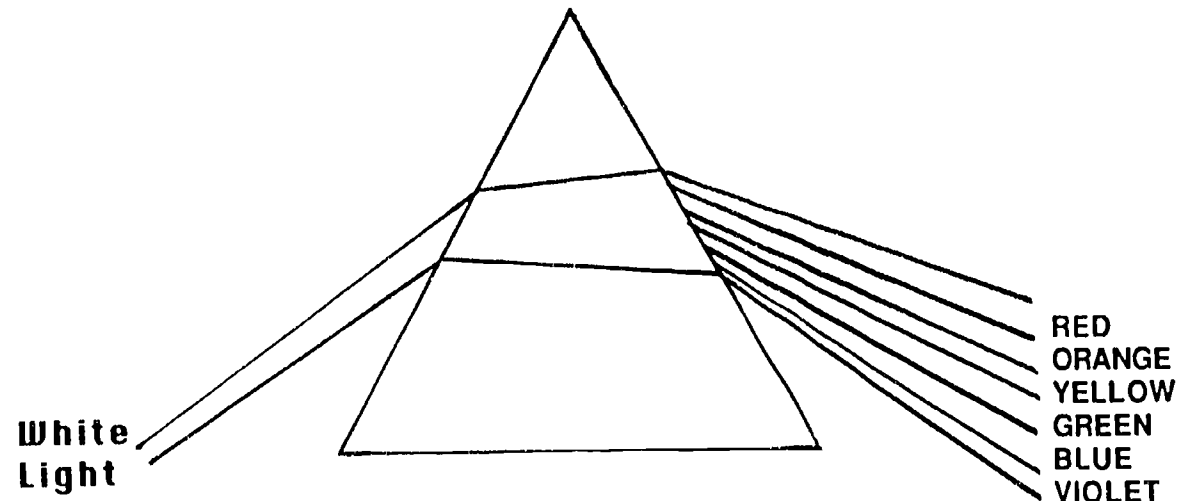
Figure 2-27 Light passing through a prism
