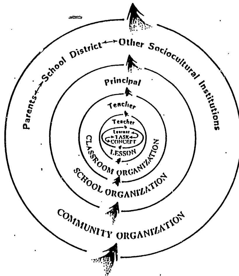
Figure 4 Embedded Contexts.
