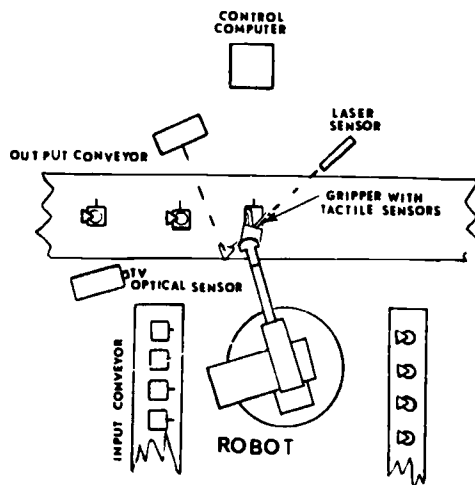
FIGURE 2 Work Cell: Robot in Work Cell With Three Sensing Systems
