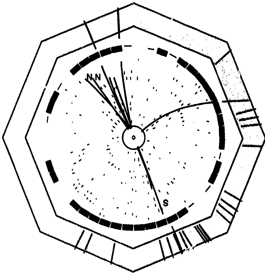
The stuff of matter. In this computer image, researchers at the Stanford Linear Accelerator capture a Z particle (center) decaying into eight subatomic particles that fan out along the red lines. (The view is looking through a barrel-shaped detector. N indicates particles leaving the north end; S indicates particles leaving the south end of the detector.)
